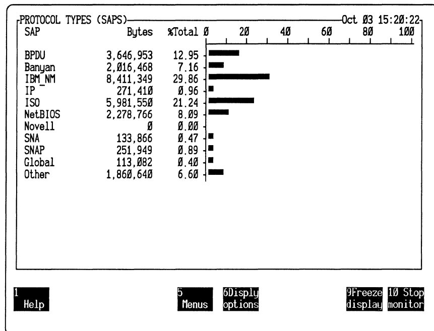
Figure 3-9. SAP Protocol Types view.
