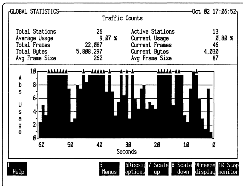
Figure 9-3. Global statistics (graphic view).
