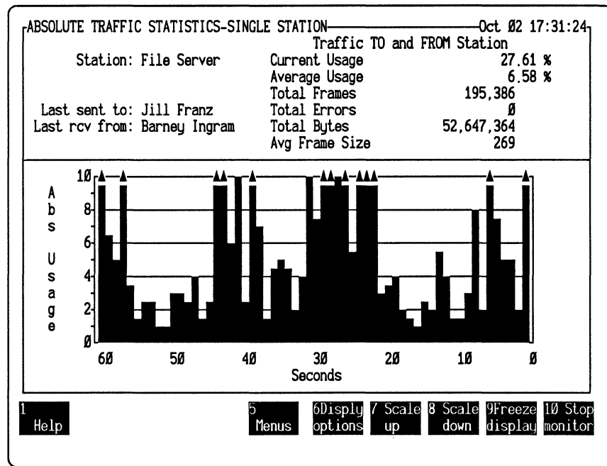
Figure 9-5. Traffic statistics for a single station (graphic view).
