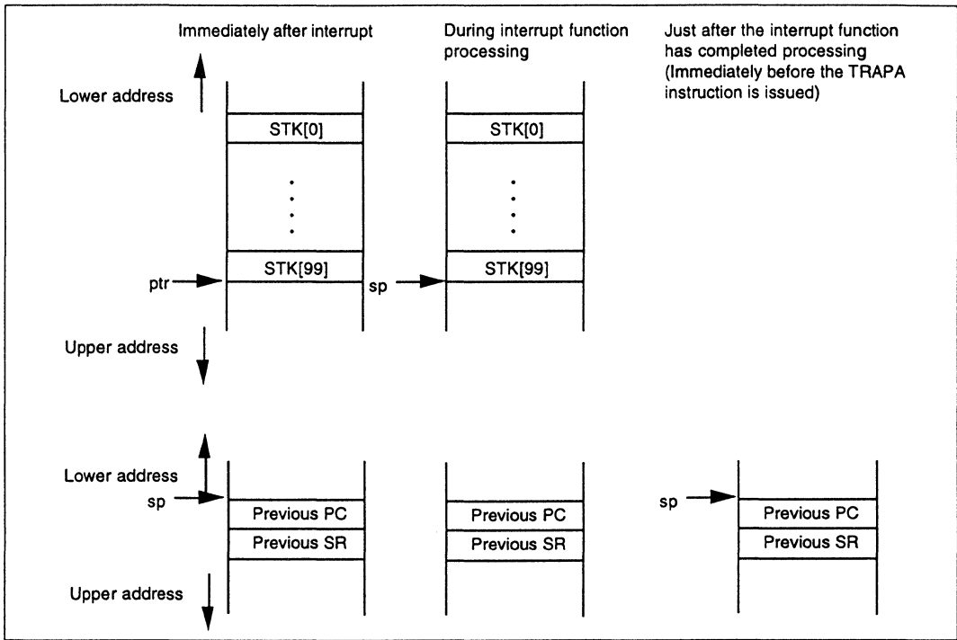
Figure 2.5 Stack Processing by an Interrupt Function
