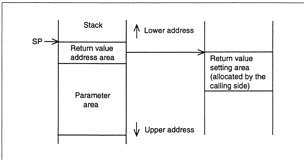
Figure 2.4 Return Value Setting Area Used When Return Value Is Written to Memory
