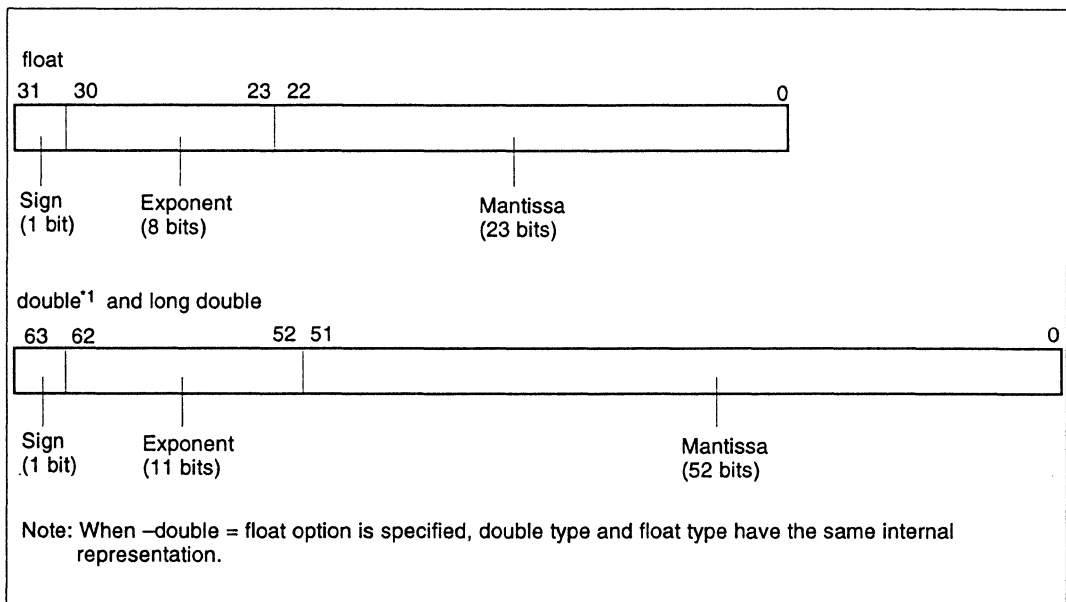
Figure A.1 Structure for the Internal Representation of Floating-Point Numbers
