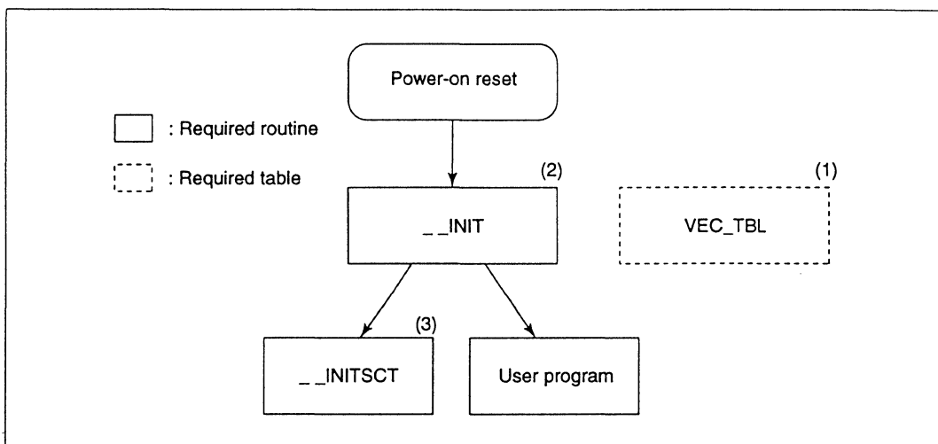
Figure 3.4 Program Configuration (No C Library Function is Used)
