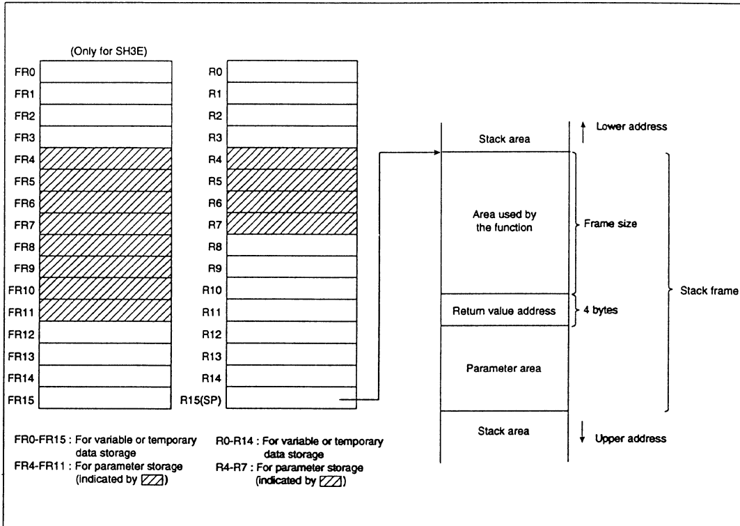
Figure C.1 Usage of Registers and Stack Area
