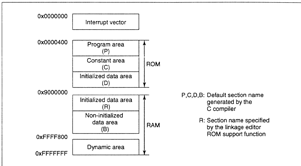
Figure 3.2 Static Area Allocation
