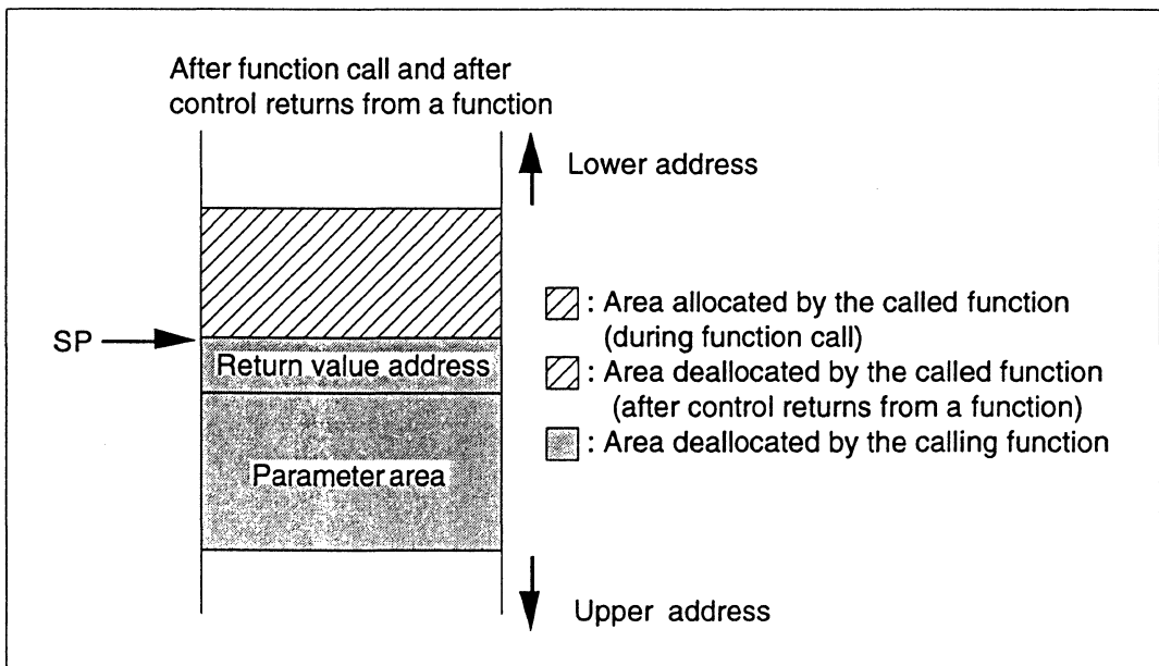
Figure 2.1 Allocation and Deallocation of a Stack Frame
