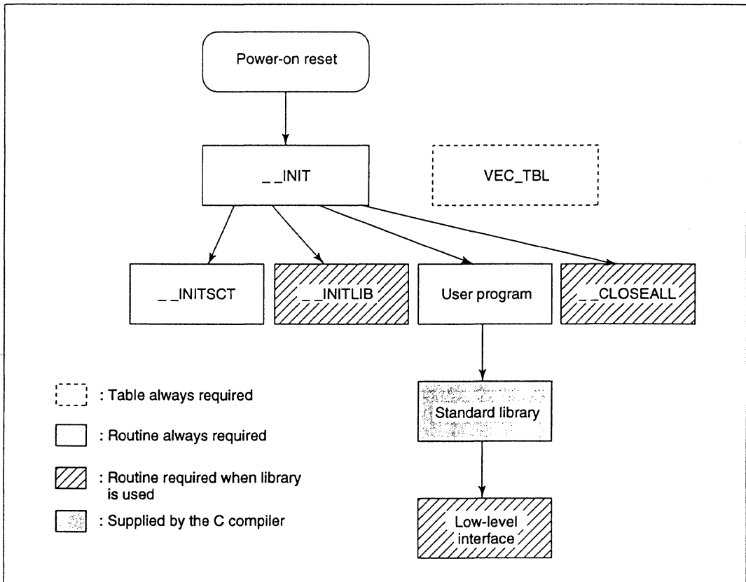
Figure 3.5 Program Configuration When C Library Functions are Used
