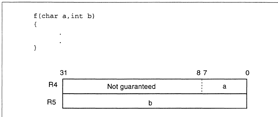
Figure 2.3 Example of Allocation to Parameter Registers
