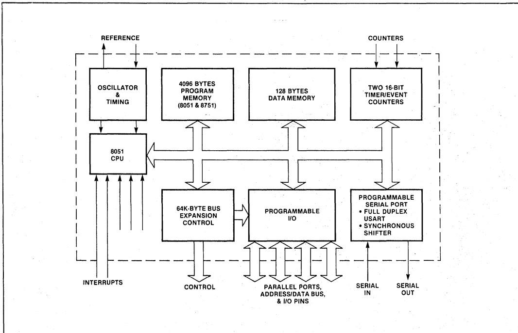
Figure 1. 8051 Block Diagram
