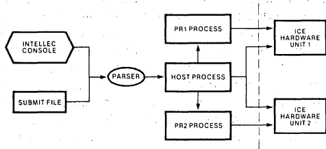
Block Diagram of Multi-ICE™ Operation
