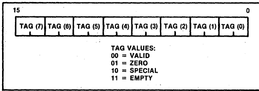
Figure 5. 8087 Tag Word
