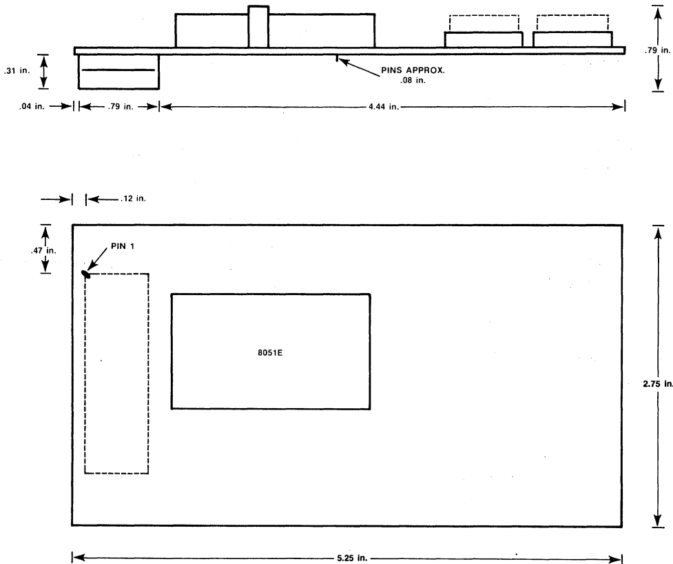
Figure 1. Dimensions
