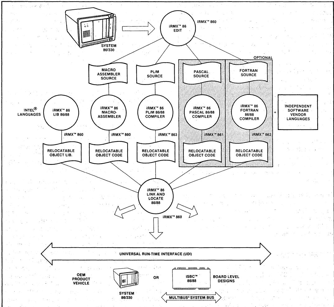
Figure 2. Software Development Process
