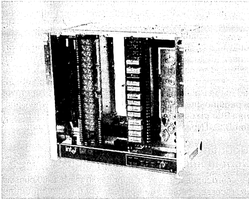
Figure 2. Small Configuration ICS 80 with iSBC 635, iCS 910 and iCS 930 Signal Conditioning/Termination Panels
