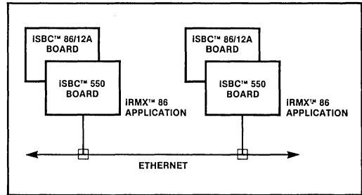
Figure 3. Ethernet Communications
