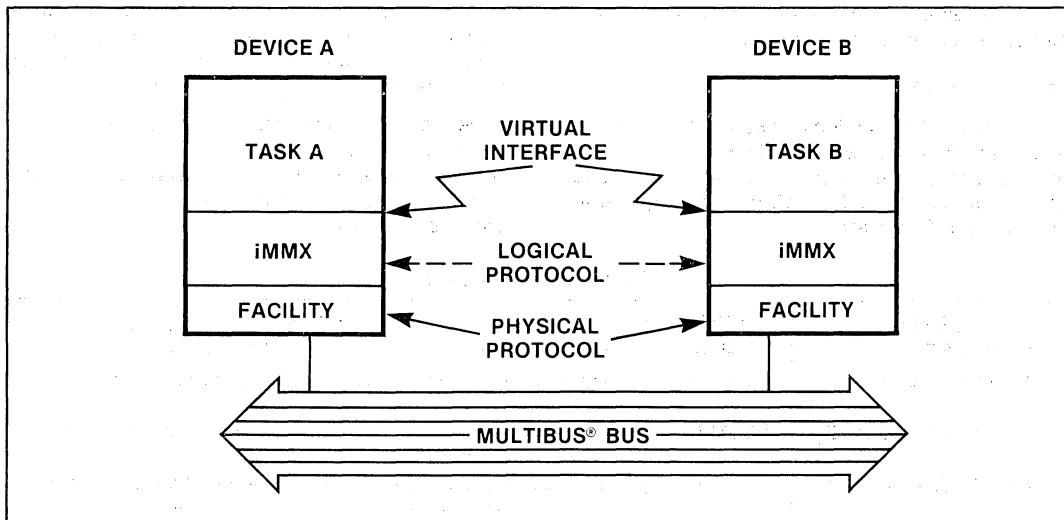
Figure 2. Inter-Device Task-to-Task Communications
