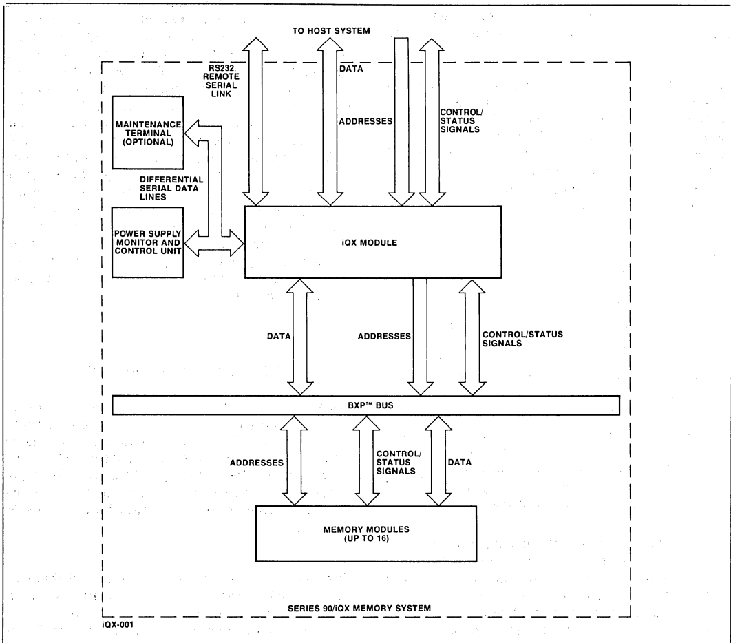
Figure 1. Series 90/iQX Memory System, Block Diagram
