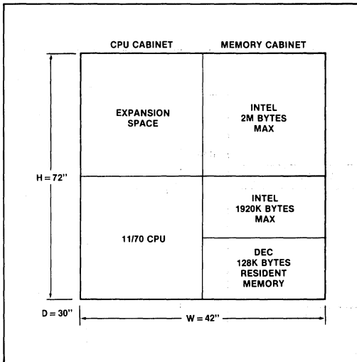
Figure 2. PDP-11/70 CPU Cabinet and in-1671 Add-On Memory Cabinet Dimensions
