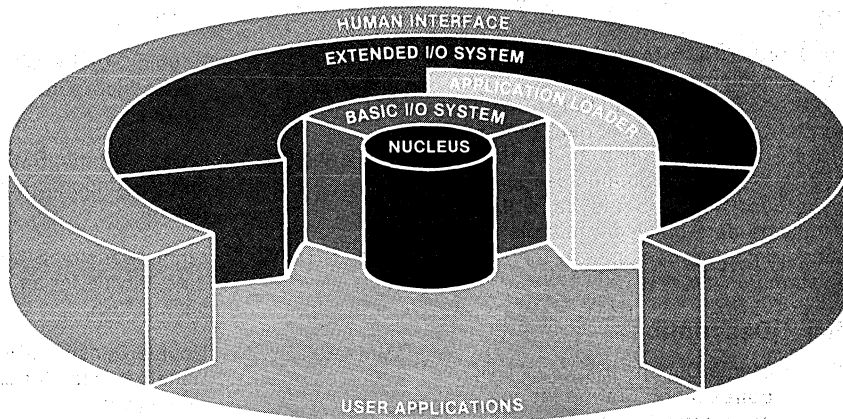
iRMX 86™ Operating System Layers
