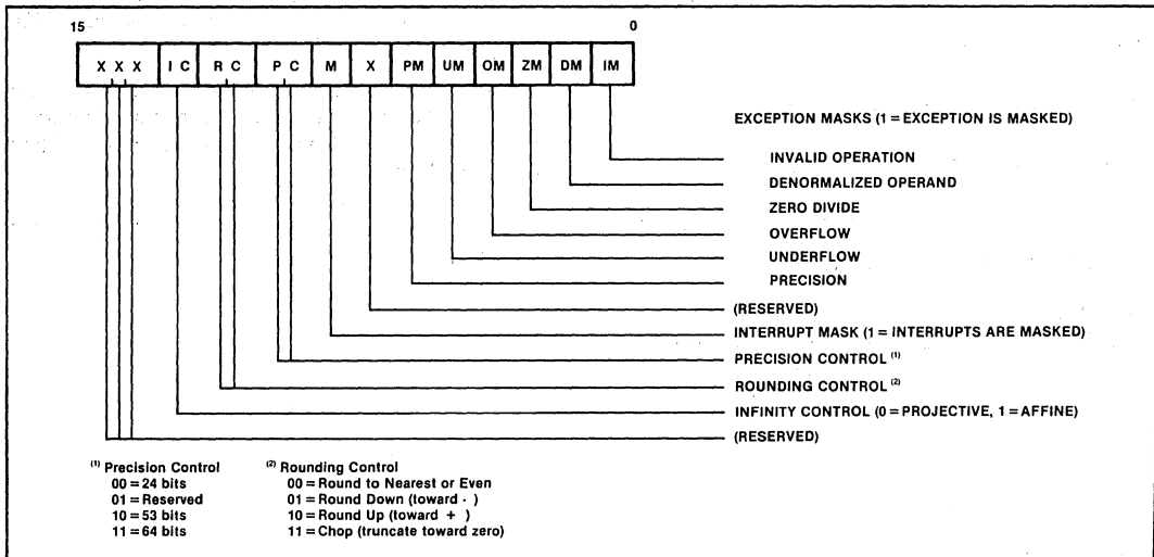
Figure 7. 8087 Control Word
