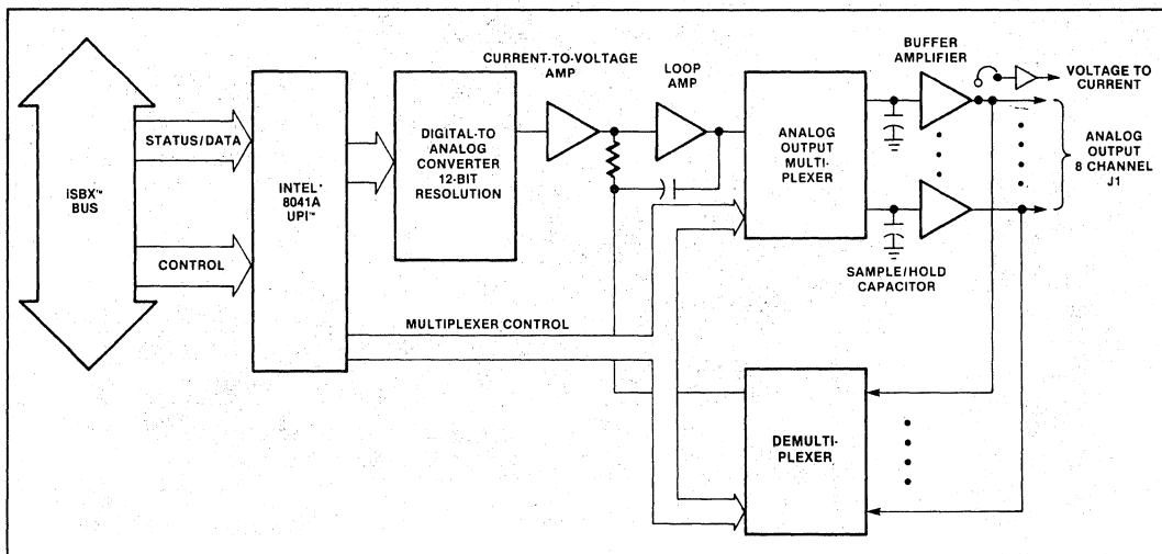
Figure 1. iSBC 328 Analog Output MULTIMODULE Board Block Diagram
