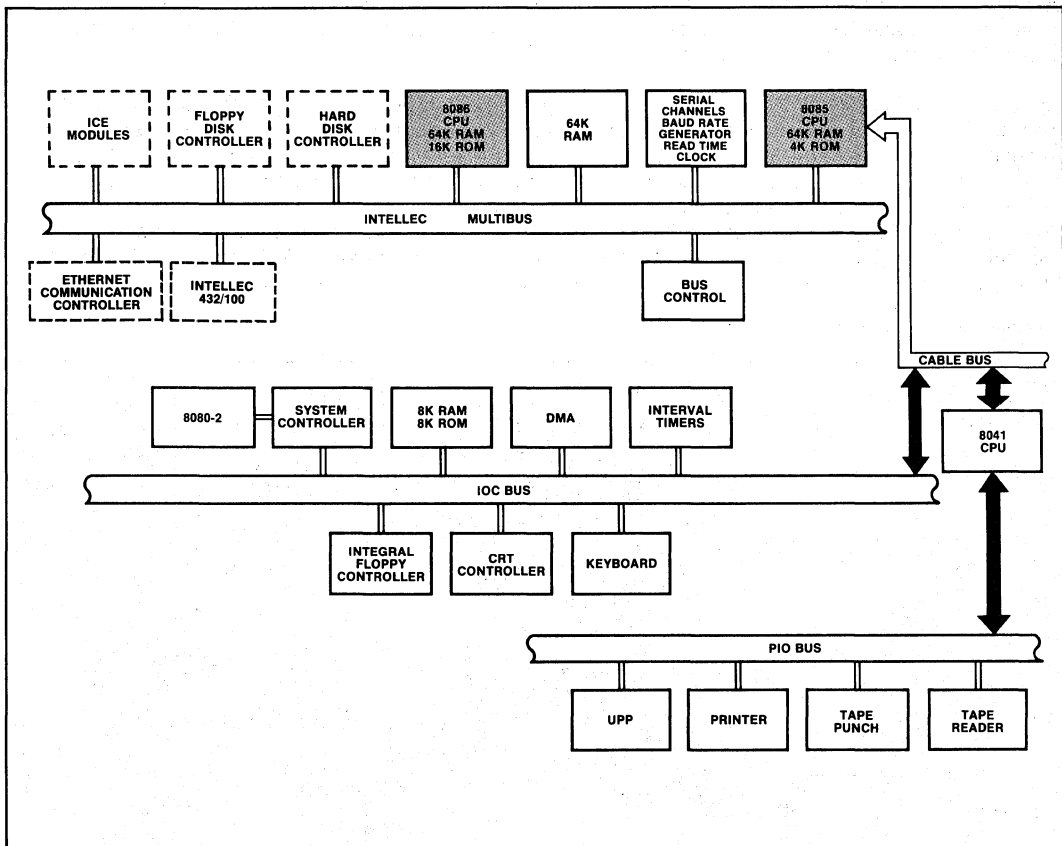
Figure 1. Model 675 DS/E Block Diagram
