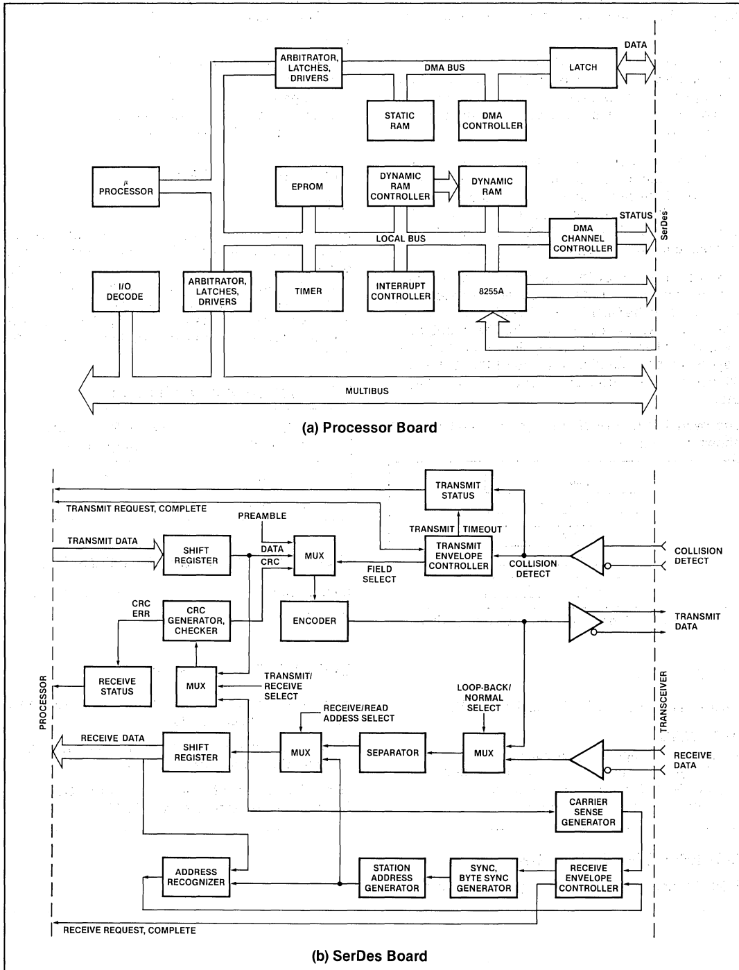
Figure 1. Block Diagram of the Ethernet Communications Controller
