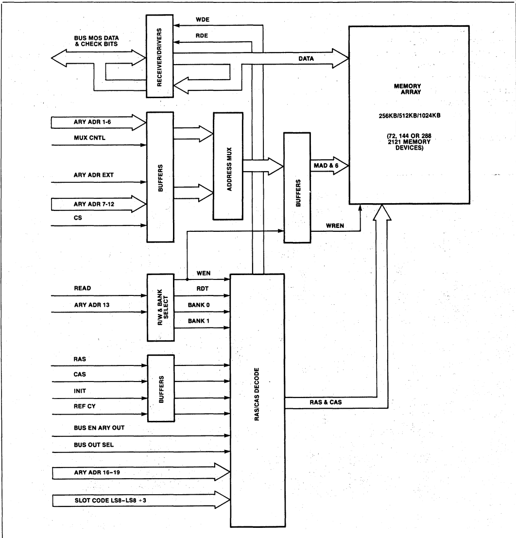
Figure 1. MU-5780 Block Diagram
