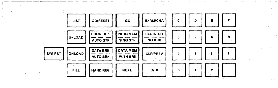
Figure 3. HSE-49 Emulator Command Keypad Organization
