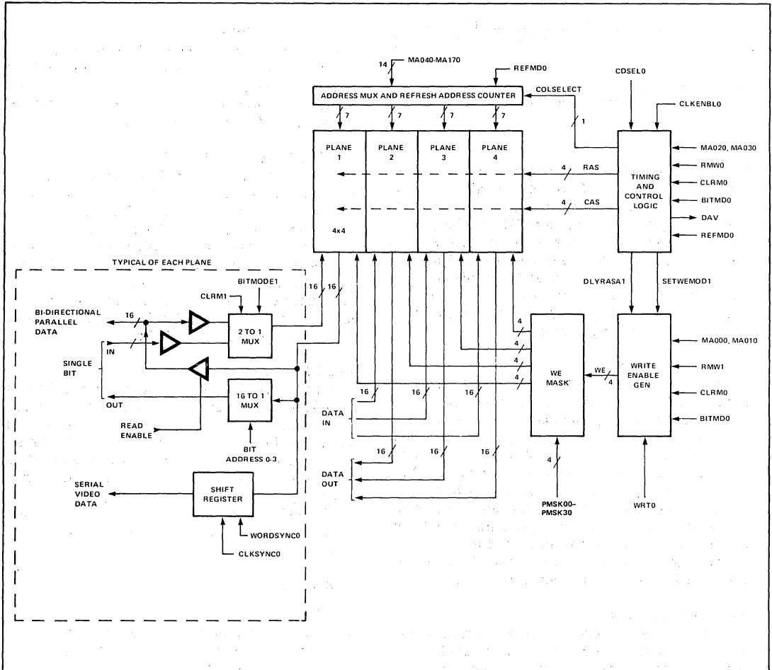
Figure 1. in-5770 Video Refresh Memory System Block Diagram
