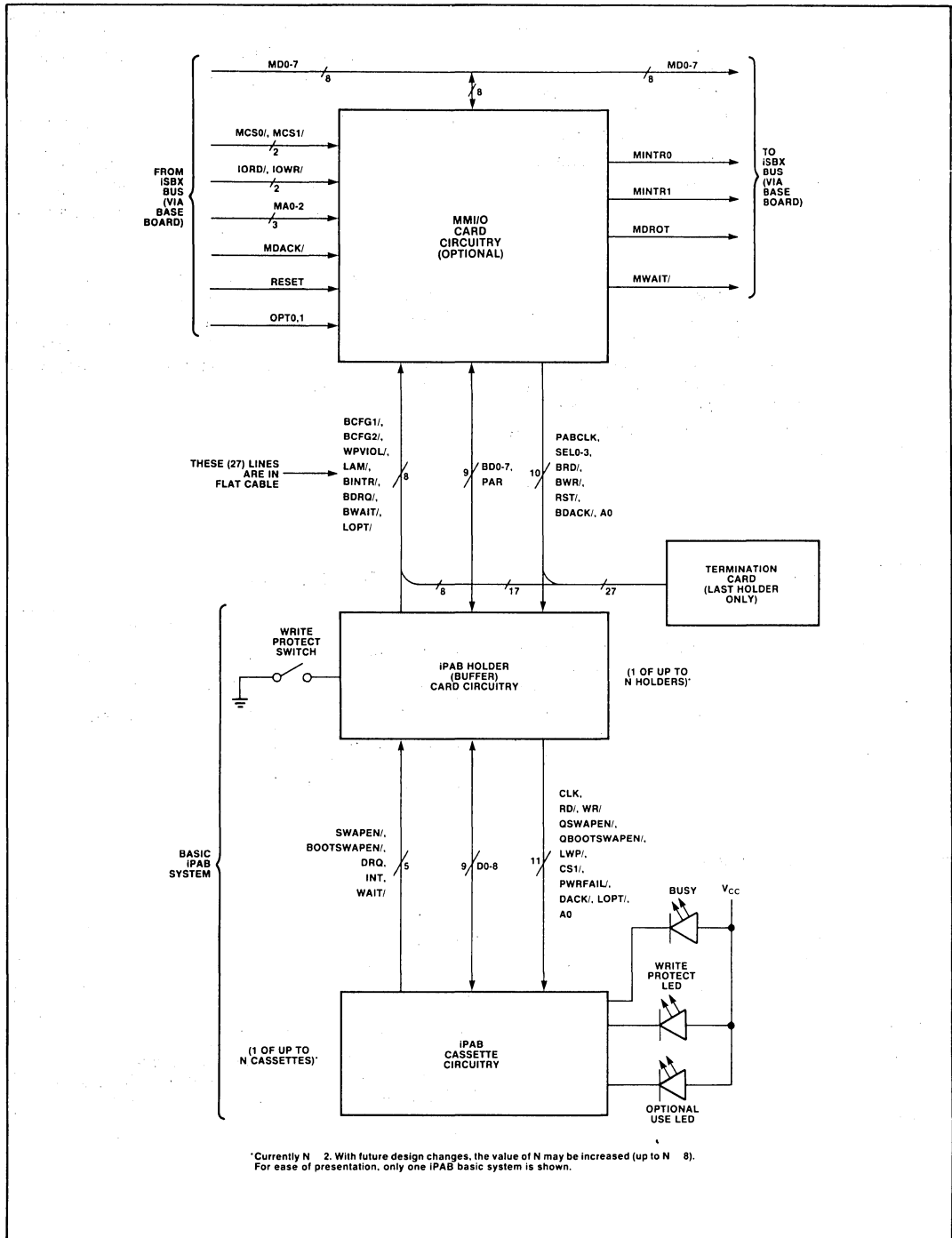
Figure 2. IPAB System Overall Block Diagram (with optional MMI/O card)
