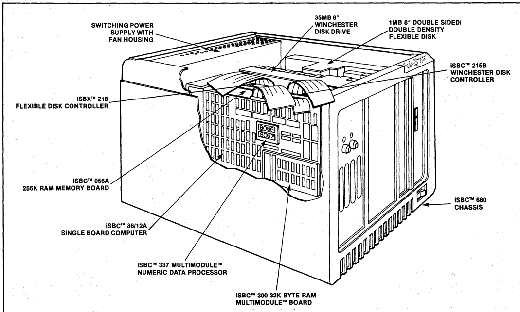
Figure 1. SYSTEM 86/330 Microcomputer System
