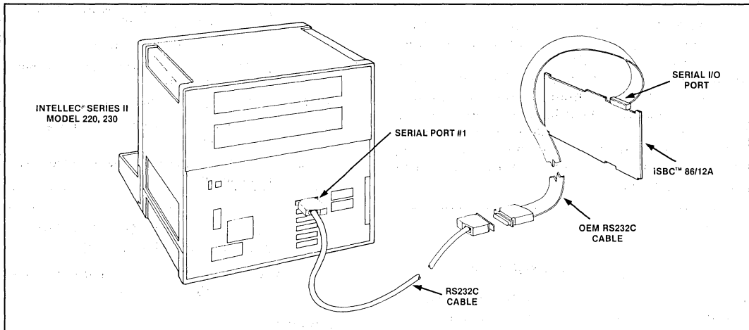
Figure 1. Intel® Series Models 220, 230 Serial Connection
