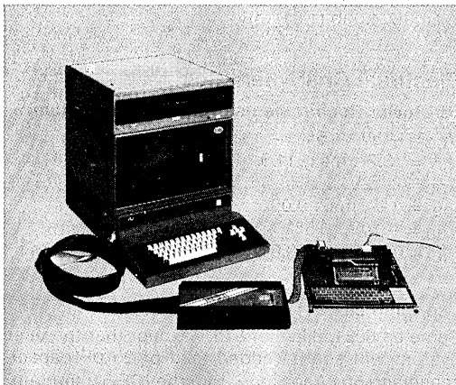
Figure 1. A Typical 8051 Development Configuration. The host system is an Intel Model 225, plus 1 megabyte dual double-density flexible disk storage. The ICE-51 module is connected to an SDK-51 system design kit.
