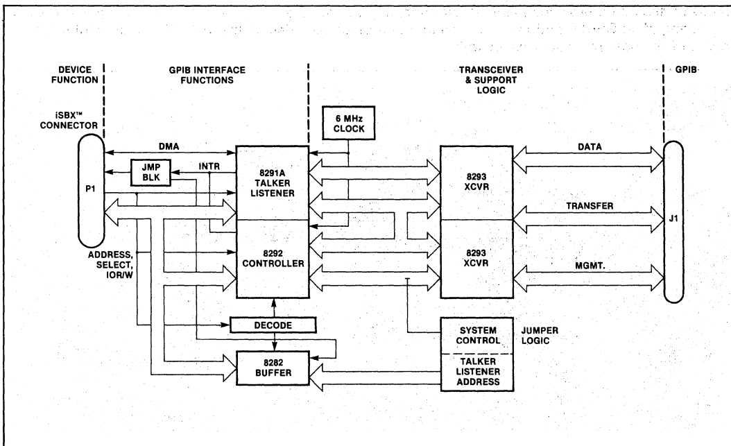
Figure 1. iSBX 488™ Multimodule Board Block Diagram
