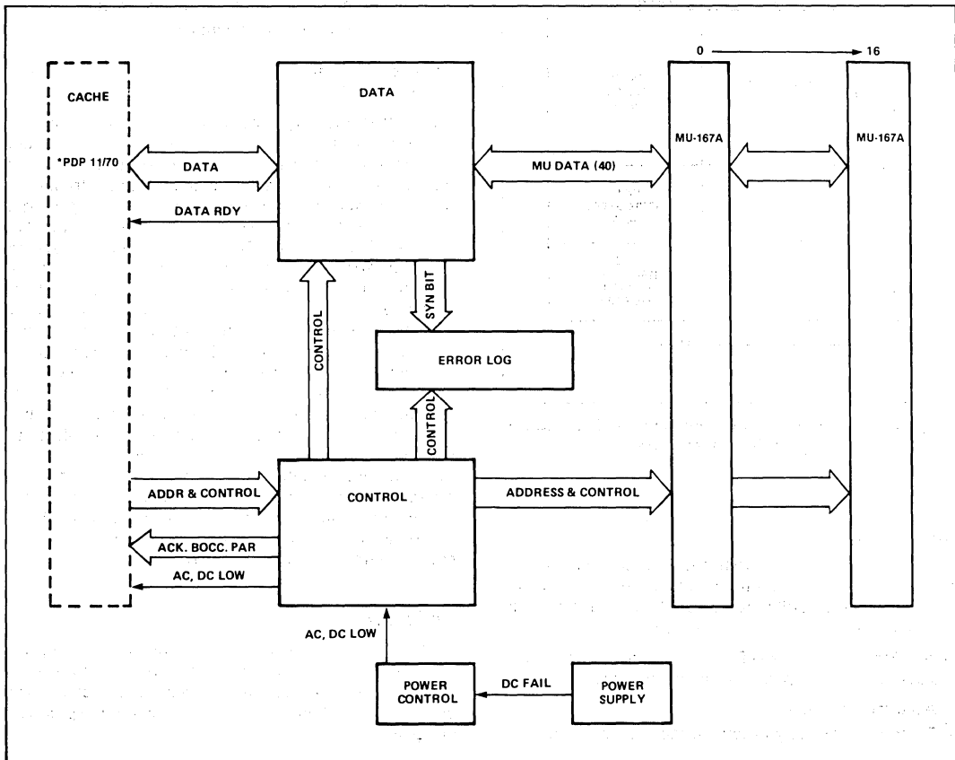
Figure 1. in-1671 Add-On Memory System Block Diagram
