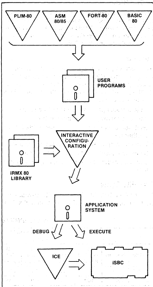
Figure 3. The System Generation Process
