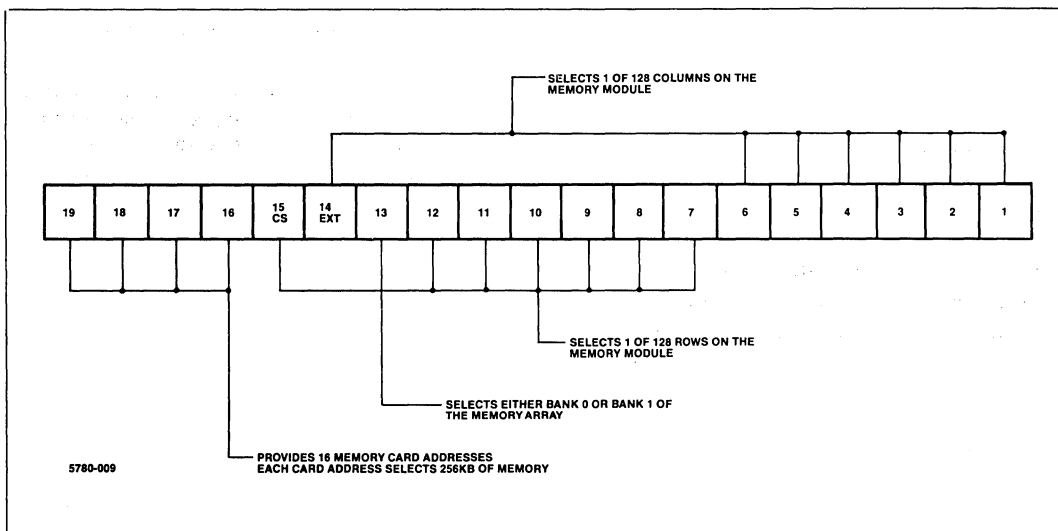
Figure 2. MU-5780 Address Configuration
