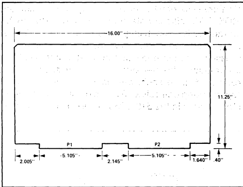
Figure 2. in-5770 Card Dimensions
