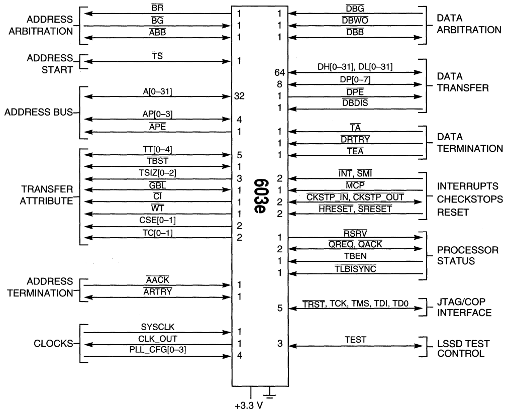
Figure 1-7. Signal Groups
