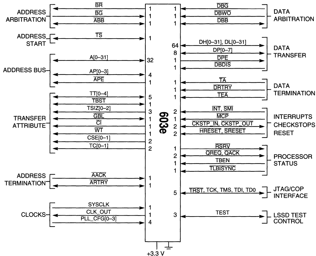
Figure 7-1. Signal Groups
