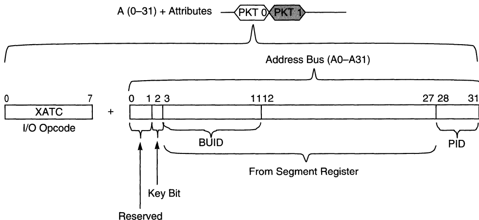
Figure C-2. Direct-Store Operation—Packet 0
