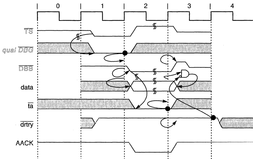
Figure 8-9. Normal Single-Beat Read Termination
