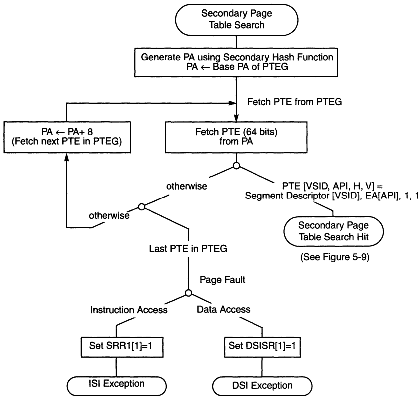
Figure 5-10. Secondary Page Table Search Flow—Conceptual Flow
