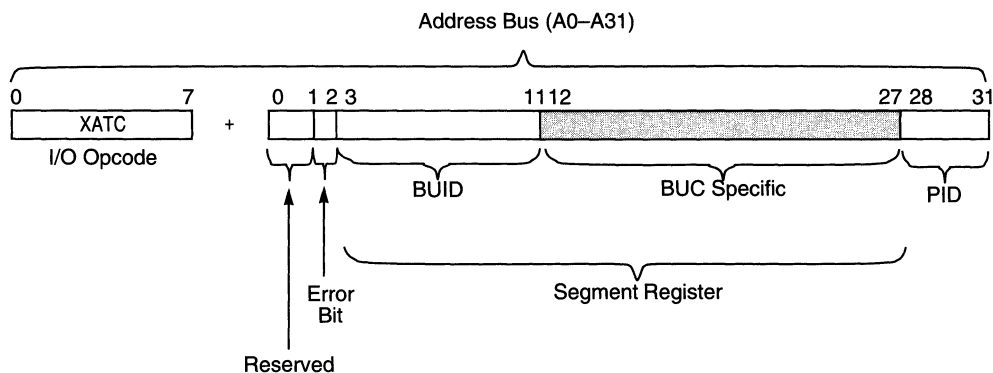
Figure C-4. I/O Reply Operation
