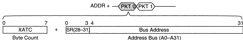
Figure C-3. Direct-Store Operation—Packet 1
