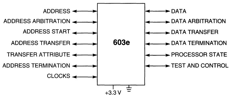
Figure 1-6. System Interface
