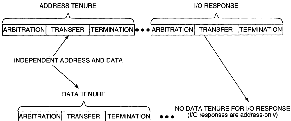
Figure C-1. Direct-Store Tenures
