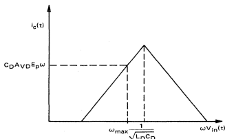
FIGURE 26 – COMPLETE RESPONSE OF DIFFERENTIATOR
