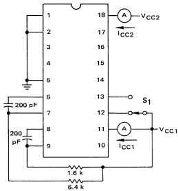
FIGURE 1 – POWER SUPPLY CURRENTS, I_{CC1} AND I_{CC2}
