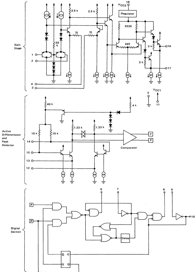
MC3470 CIRCUIT SCHEMATIC
