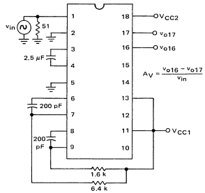
FIGURE 2 – VOLTAGE GAIN, BANDWIDTH, OUTPUT VOLTAGE SWING
