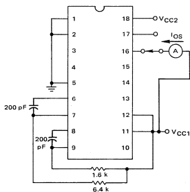
FIGURE 4 – AMPLIFIER OUTPUT SINK CURRENT, PINS 16 AND 17
