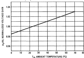
FIGURE 16 – NORMALIZED VOLTAGE GAIN (A_V/A_V 25^\circ\text{C}) versus TEMPERATURE
