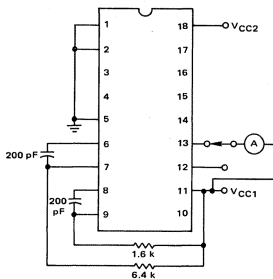
FIGURE 6 – DIFFERENTIATOR OUTPUT SINK CURRENT, PINS 12 AND 13
