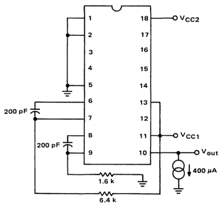
FIGURE 9 – DATA OUTPUT VOLTAGE HIGH, PIN 10
