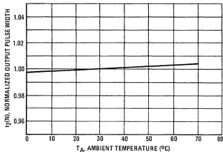
FIGURE 19 — NORMALIZED OUTPUT PULSE WIDTH, t_2/t_2 25°C
