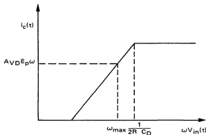
FIGURE 25 – RESPONSE OF DIFFERENTIATOR USING ONLY C_D
