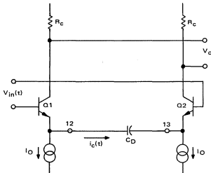
FIGURE 24 — ACTIVE DIFFERENTIATOR NETWORK
