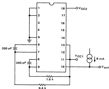
FIGURE 10 – DATA OUTPUT VOLTAGE LOW, PIN 10
