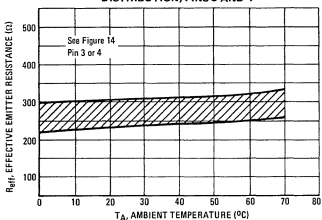
FIGURE 21 — EFFECTIVE EMITTER RESISTANCE DISTRIBUTION, PINS 3 AND 4
