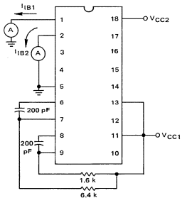
FIGURE 3 – AMPLIFIER INPUT BIAS CURRENT, I_{IB}
