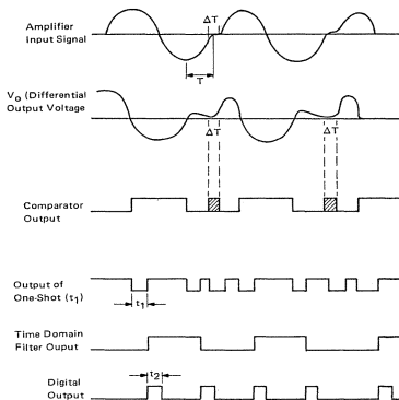
FIGURE 28 — WAVEFORMS THROUGH THE READ CIRCUIT
