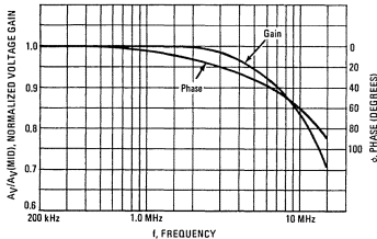
FIGURE 17 — PHASE AND NORMALIZED VOLTAGE GAIN versus FREQUENCY
