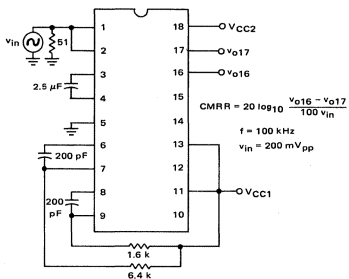
FIGURE 5 – AMPLIFIER COMMON MODE REJECTION RATIO, CMRR
