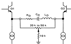
FIGURE 27 – PEAK SHIFT COMPENSATION
