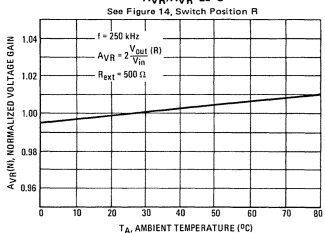
FIGURE 20 — NORMALIZED VOLTAGE GAIN, A_{VR}/A_{VR} 25°C
