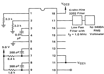
FIGURE 22 — DIFFERENTIAL NOISE VOLTAGE
