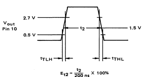
FIGURE 11 – DATA OUTPUT RISE TIME, t_{RLH} DATA OUTPUT FALL TIME, t_{THL} TIMING ACCURACY MONO #2, E_{t2}
