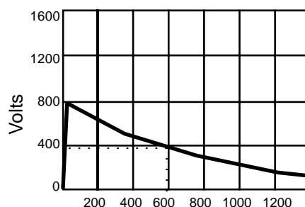
10 by 560 – 800 Volts FCC – Metallic Surge
