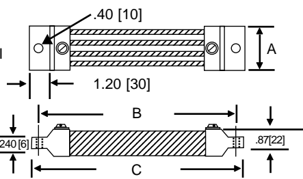
Figure 4 Horizontal Mount
