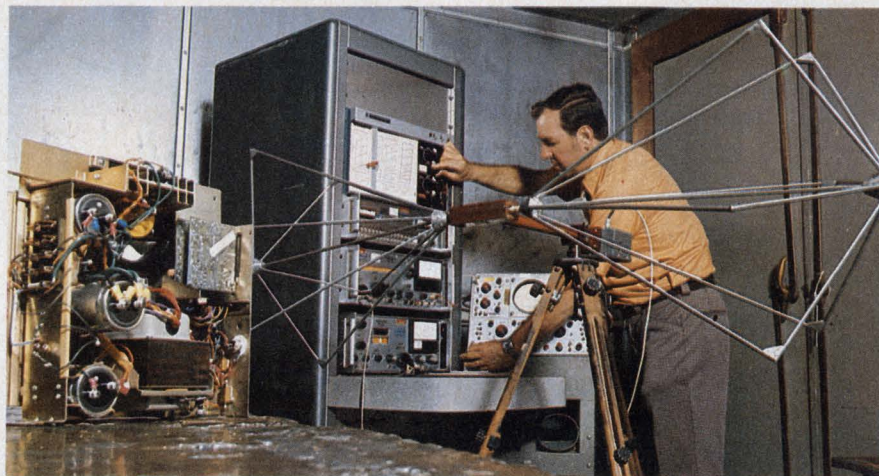
Radiated interference from a display-terminal power supply being measured for a customer at Sanders Associates, Nashua, NH, electromagnetic-compatibility test facility. Measurements are being made between 20 and 200 MHz.
