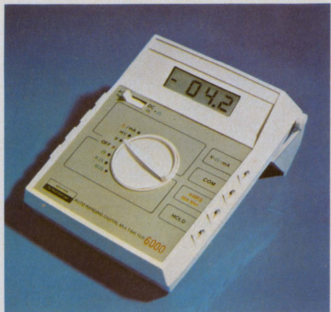
Over 200 hours of battery life marks the Weston 6000, a field unit that uses LCDs. A "hold" feature lets you concentrate on the measurement, not the reading.
