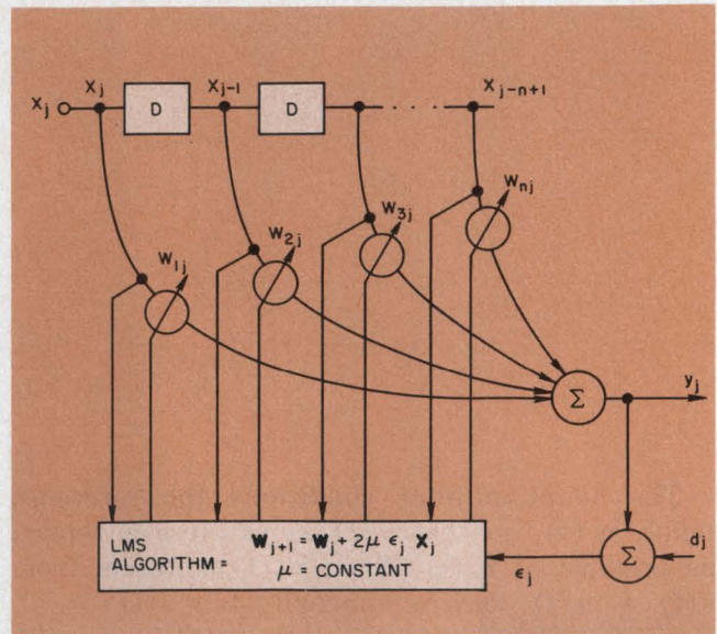
5. For broadband signals, the adaptive technique takes the shape of a tapped delay line, or variable-weight transversal filter.
