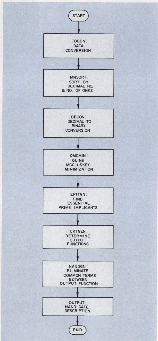
1. The ROMGEN program sequentially steps through subroutines to input the data, minimize the minterms and generate output descriptions of the NAND gates.
