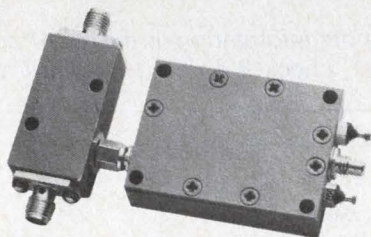
Output connector of new fully TTL compatible switch driver (right) mates with the SMC connector on the new HP fast PIN diode switch.
