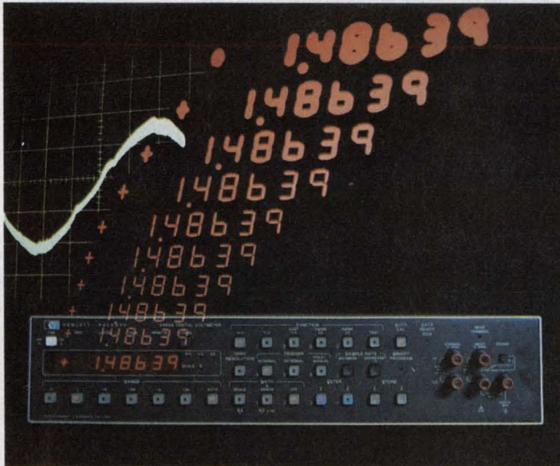
With internal \mu Ps and memories, systems DMMs are growing in sophistication. This Hewlett-Packard unit is the first to offer a removable reference module.
