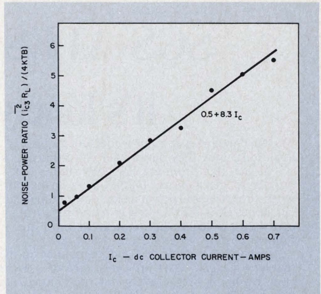
6. An empirical straight line can be fitted to represent the transistor's noise-power ratio vs its collector current.
