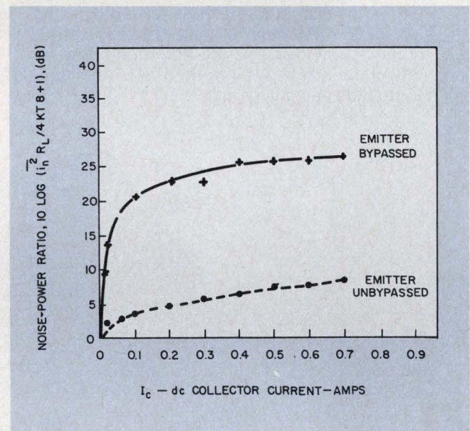
7. Plots of noise-power ratio, with and without emitter degeneration, show that an improvement of about 18 dB results with degeneration.
