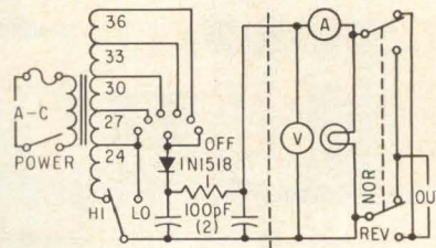
POWER SUPPLY provides wide range of voltages for testing breadboard transistor circuits—Fig. 1
