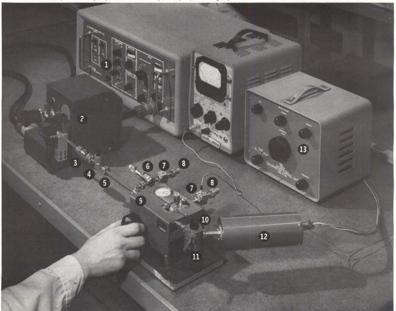
TRG test bench components: the only complete line for W-band — (75-110 Gc) — (WR-10 waveguide)
