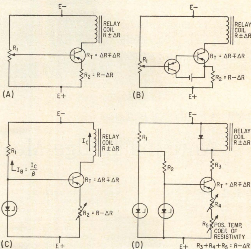
CIRCUITS (A) and (B) compensate for relay resistance variations, circuit (C) for supply voltage variations and (D) for ambient temperature—Fig. 1
