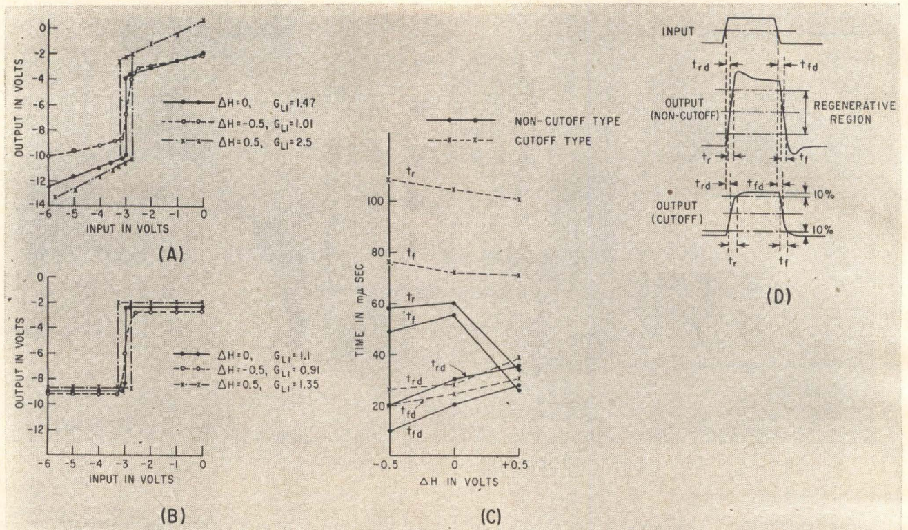
STATIC CHARACTERISTICS of non-cutoff Schmitt trigger (A) and cutoff Schmitt trigger (B); switching characteristics of Schmitt trigger circuits (C) along with definitions of abbreviations (D)—Fig. 3
