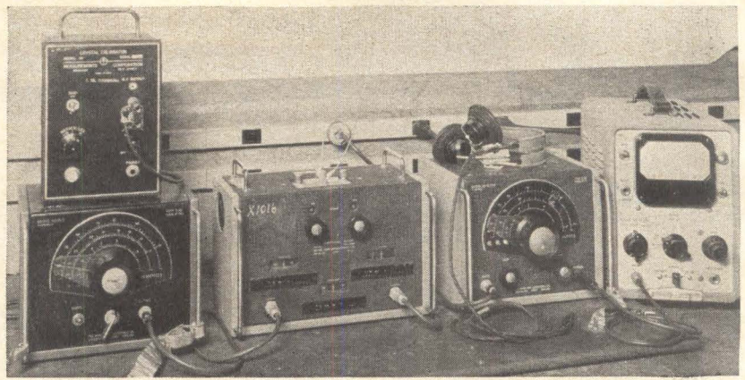
TYPICAL TEST setup with standing-wave indicator at right
