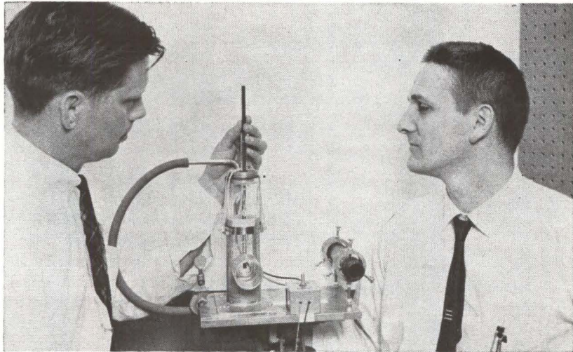
TV TRANSMITTER. Developers examine assembly holding gallium arsenide diode, located at bottom of black rod. Beam is emitted from circular window in lower half of transmitter
