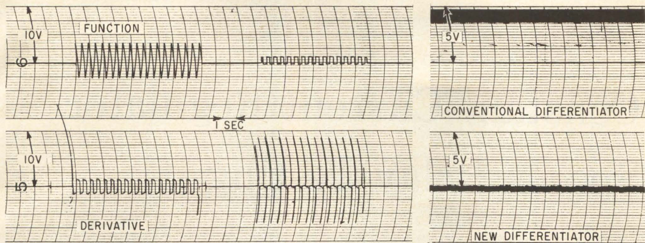
DIFFERENTIATION OF TRIANGULAR and square waves with improved model (left) and comparison of differentiator noise (right)—Fig. 2
