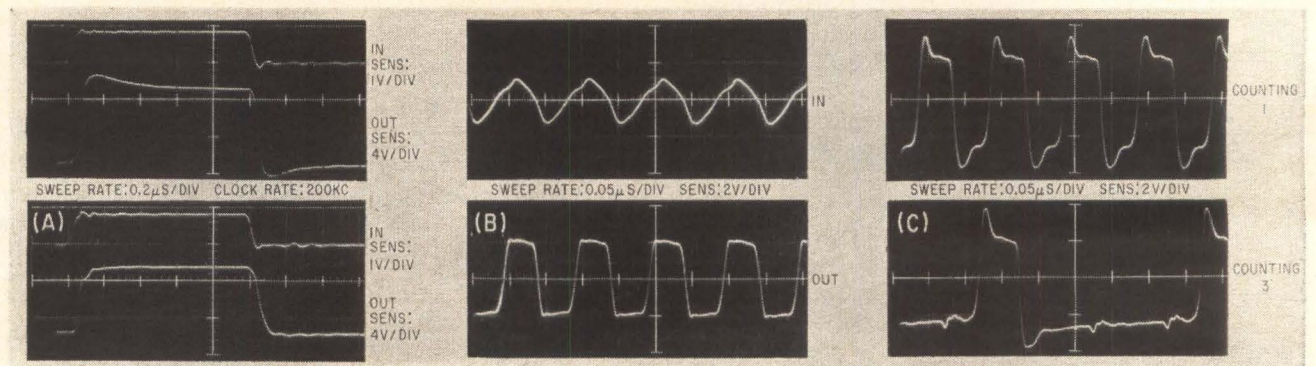
INPUT-OUTPUT WAVEFORMS of noncutoff (top) and cutoff (bottom) types of Schmitt trigger circuits (A); input-output waveforms of noncutoff Schmitt trigger circuit used as pulse shaper at clock rate of 10 Mc (B); output waveforms of noncutoff monostable multivibrator at trigger rate of 10 Mc (C)—Fig. 4
