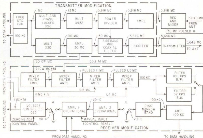
MODIFIED transmitter and receiver of the AN/FPS-16. Other modifications were made in the data-handling system
