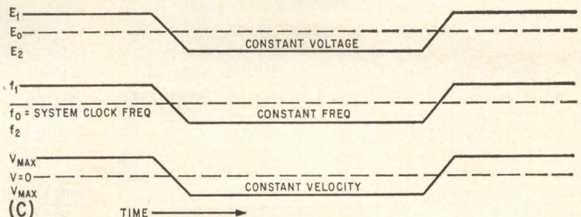
DIRECTION SENSOR (A) of simulator. Encircled portions of timing diagram (B) show that only one SV pulse is enclosed by gates. In (C), voltage E controls oscillator frequency f , which produces simulated target velocity V —Fig. 3
