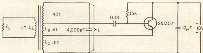
FINAL DESIGN of 122-Kc oscillator. Transformer is No. 30 wire wound on a Ferroxcube core—Fig. 3
