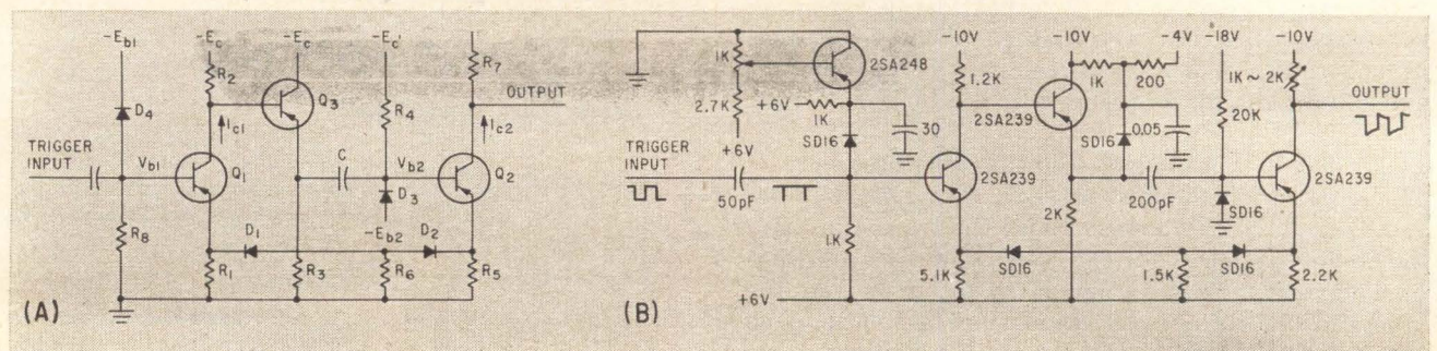
BASIC CIRCUIT of noncutoff monostable multivibrator (A) and experimental circuit (B)—Fig. 5
