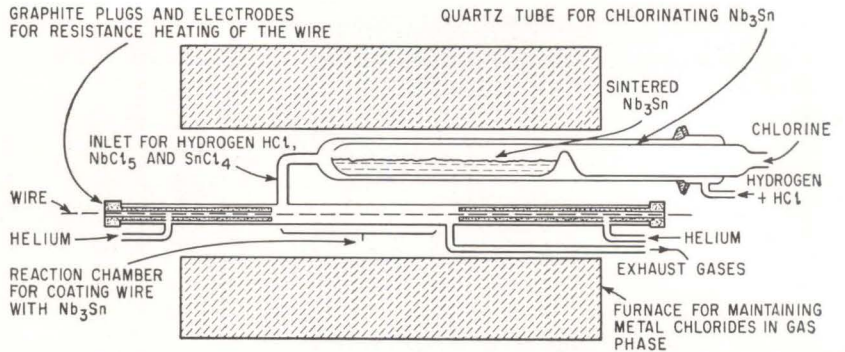
NIOBIUM-TIN is deposited on wire substrate with irreversible gas-phase transport technique. When cooled to superconductivity, wire can carry current at a density of ½ million amps per cm 2 in a 90,000 gauss field
