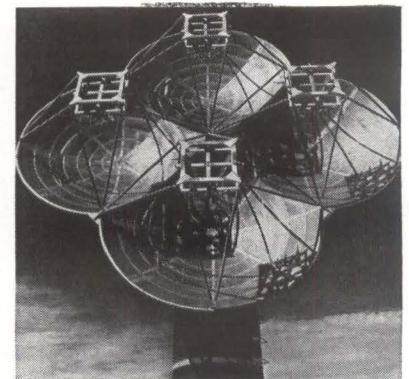
ARRAY of reflectors is about 20 feet in diameter
