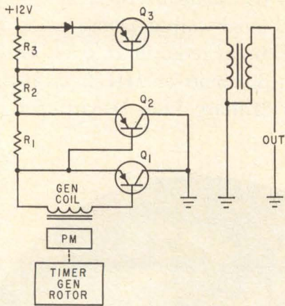
ROTATING permanent magnet switches transistors on and then off, interrupting current in primary of output transformer to generate ignition pulse—Fig. 1
