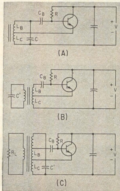
HARTLEY CIRCUIT (A), and method of isolating tank circuit (B) or transforming load to a desired value (C)—Fig. 1
