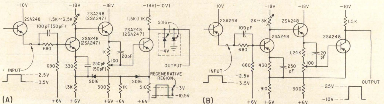
EXPERIMENTAL NONCUTOFF Schmitt trigger circuit (A) compared to cutoff type (B)—Fig. 2
