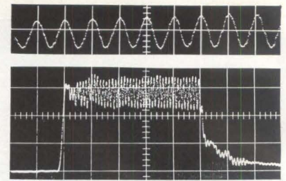
MICROWAVE oscillation in GaAs block are shown in lower trace (divisions are 2 nsec horizontally and 0.23 amp vertically). Upper trace shows oscillation magnification (IBM)
