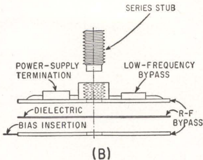
SIMPLIFIED tunnel diode preamplifier circuit (A) and its physical arrangement (B). Three-port circulator coupled L-band amplifier (C)—Fig. 3
