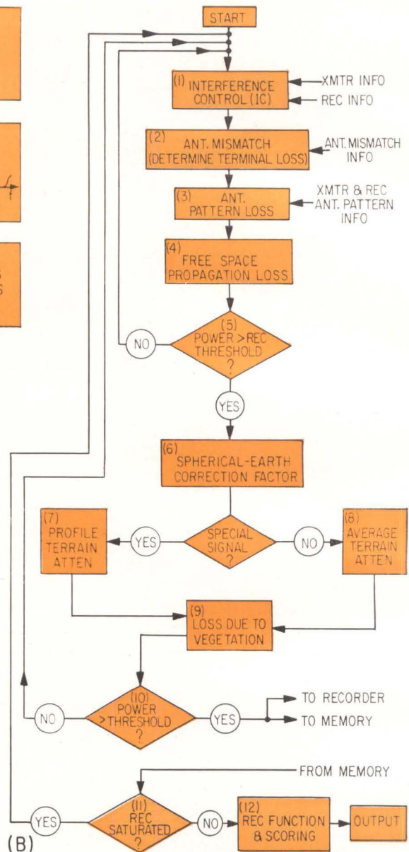
MATHEMATICAL MODEL of the electromagnetic environment of the communications system shown in the upper row of blocks (A). Computer programming is shown in (B) and the spectrum of the signals presented to the computer program that simulates the receiver demodulator is shown in (C)—Fig. 15
