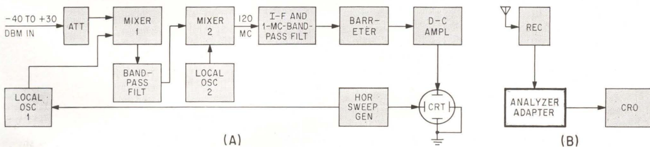
POWER-SENSING spectrum analyzer (A) produces display of input power versus frequency (GE Light Military Electronics Dept.). The adapter unit in (B) is used with a lab cro to make up a spectrum analyzer (Pentronix)—Fig. 11
