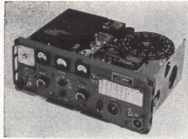
LINEAR amplifier portion of Army's new AN/GRC-106 ssb transceiver is typical of trend towards smaller high-power radios. This unit develops 400 watts
