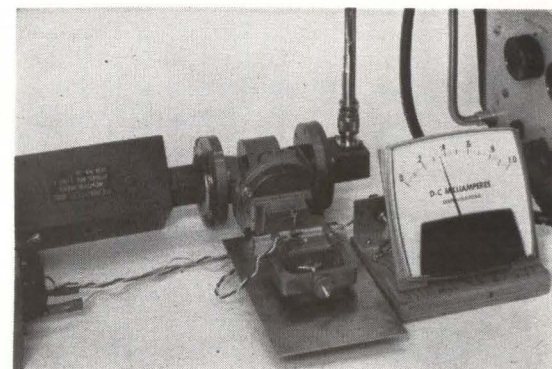
TUNNEL DIODE six-gigacycle waveguide amplifier
