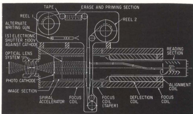
TELEVISION information storage tube including tape and optical systems is completely reusable and consumes only operating power—Fig. 1
