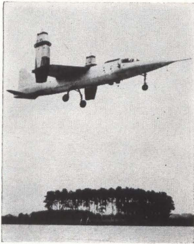
GERMANY is developing the VJ 101, a six-jet vertical takeoff and landing plane that could replace the F-104G in the 1970's
