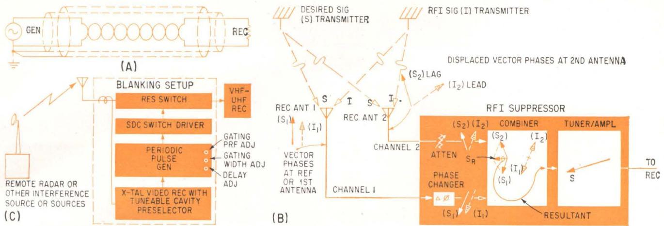
CABLE GROUNDING scheme (A) grounds outer shield at more than one point, whereas inner shield is grounded at only one end. Phase-selective action (B) can be used to suppress an rfi signal (Pioneer Electric & Research). Blanking setup (C) is used to protect vhf-uhf receiver from high-power radar pulses (RMS Engineering)—Fig. 21
