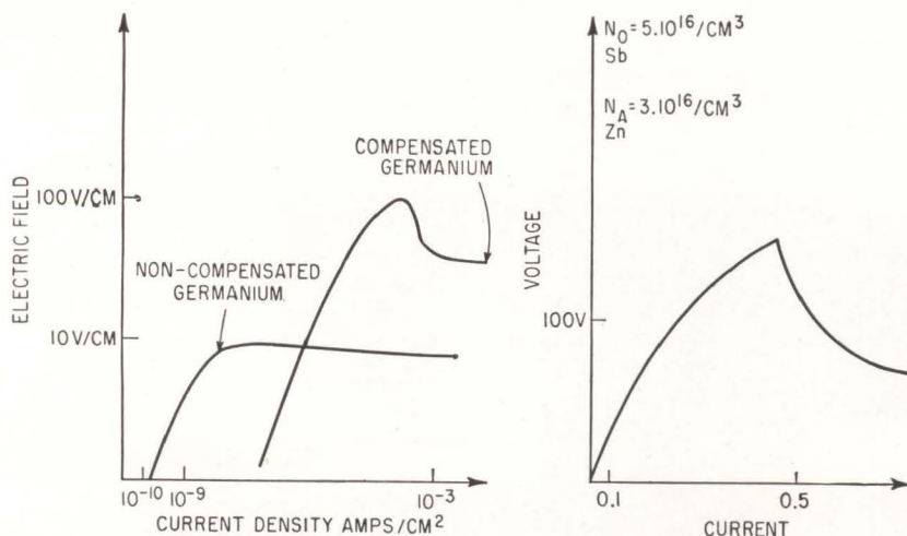
GERMANIUM CRYOSAR characteristics, left, shown for compensated and uncompensated unit. Right, I-V characteristic for germanium cryosar doped with zinc and compensated with antimony (Zylbersztein)—Fig. 1
