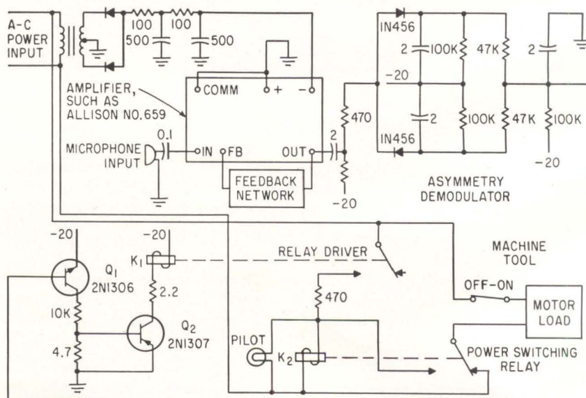
DEMULATOR for asymmetry envelope, in upper right hand corner of circuit diagram, is heart of system—Fig. 3
