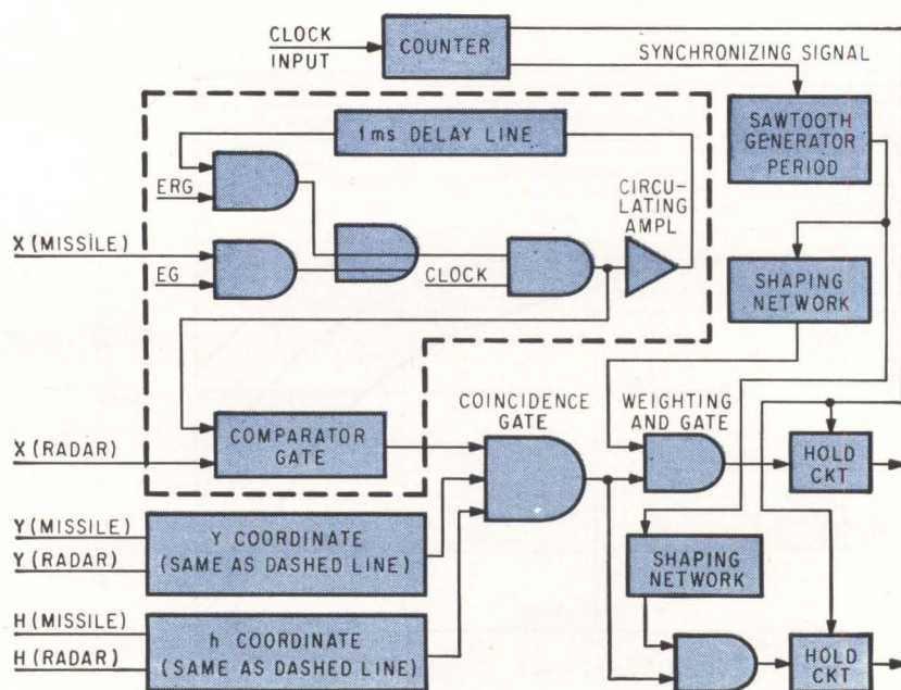
MISSILE WAKE radar return simulator is based on the estimated maximum length of the wake decay time—Fig. 6
