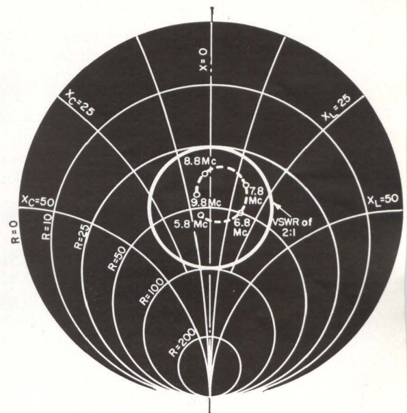
MEASURED input impedance of 5.5 to 11-Mc filter, multicoupler terminated in 50-ohm resistive load, remaining filters are detuned at least 0.7-Mc—Fig. 3
