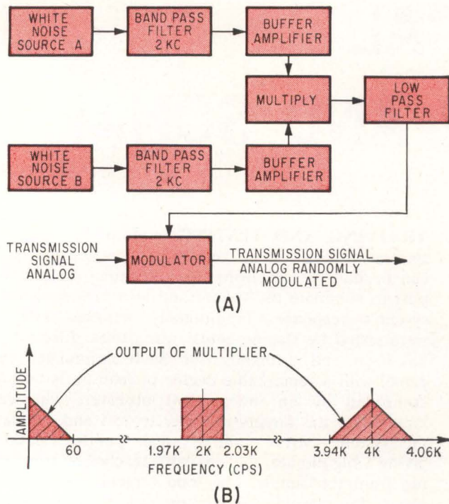
RANDOM NOISE generation system (A) is a requirement of realism; idealized spectrum (B) of system—Fig. 2
