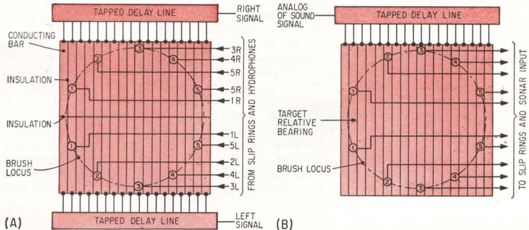
STEERABLE sonar array switching system (A) can be sophisticated by use of inverse compensating switch (B) for properly simulated signal delays in water—Fig. 4
