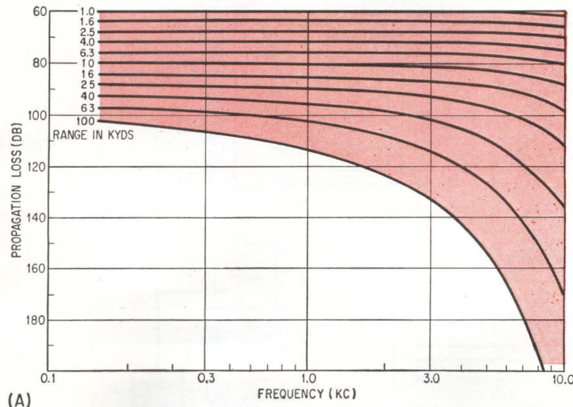
UNDERWATER SOUND in a nominal direct path propagation loss as a function of frequency (A). Range attenuation potentiometer (B) combines both spreading and absorption loss in a single unit—Fig. 5
