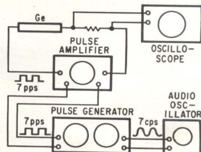
TEST CIRCUIT used for measuring effects of chemicals on oscillistor frequency and waveshape—Fig. 1
