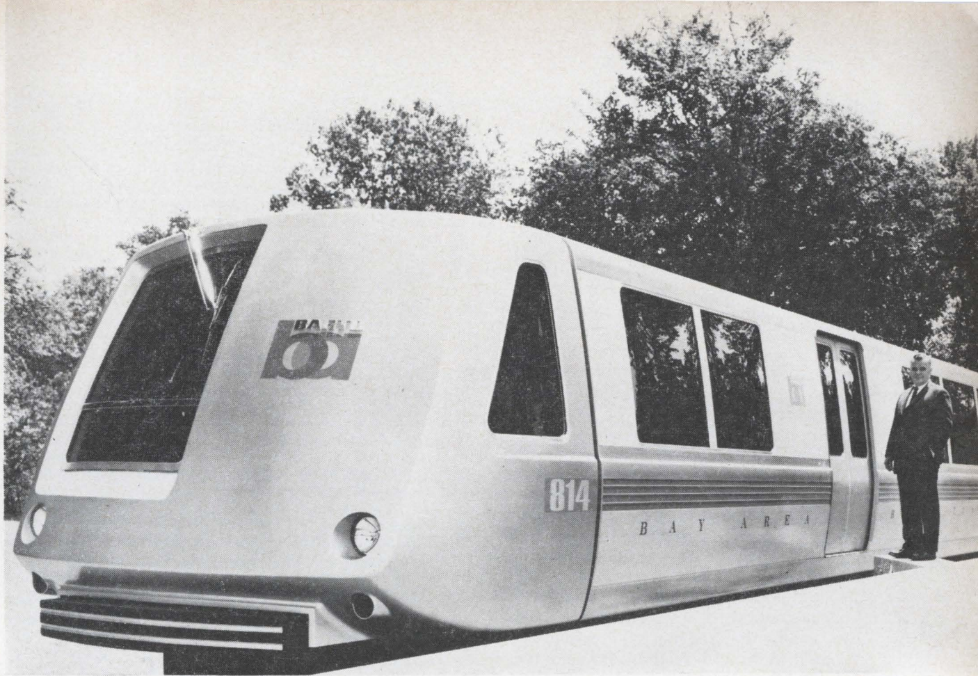
Prototype of rapid-transit car for the BARTD system. It is 72 feet long, air-conditioned, and carries 70 riders who can look out through tinted windows as they relax in upholstered comfort. The car runs on a wide-gauge 5½-ft. track (standard gauge is 4 ft. 8½ inches) for greater stability and a smoother ride. The detachable front section, or pod, carries all the electronic equipment and the one crewman aboard the train. The exact specifications of the pod will depend on the control system chosen after the test period on the Mt. Diablo track.
