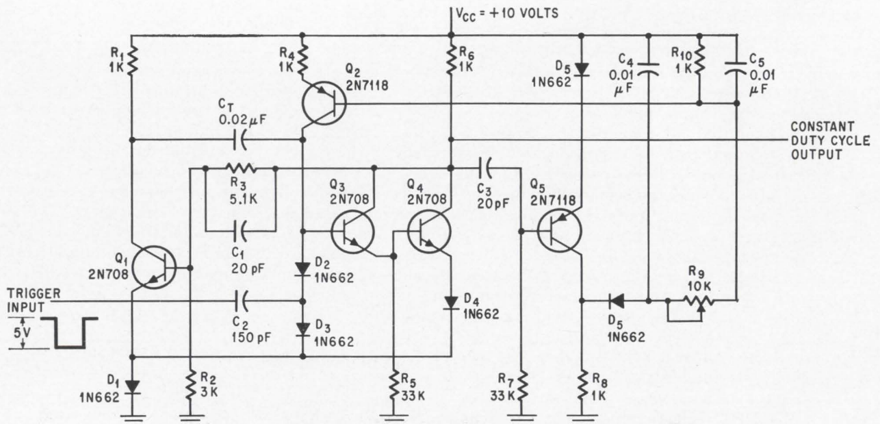
Circuit diagram of pulse generator. Q_1 , Q_3 and Q_4 form multivibrator 1. Multi 2 consists of Q_5 only. The integrator consists of R_8 and C_4 , and Q_2 is the voltage-to-current converter.
