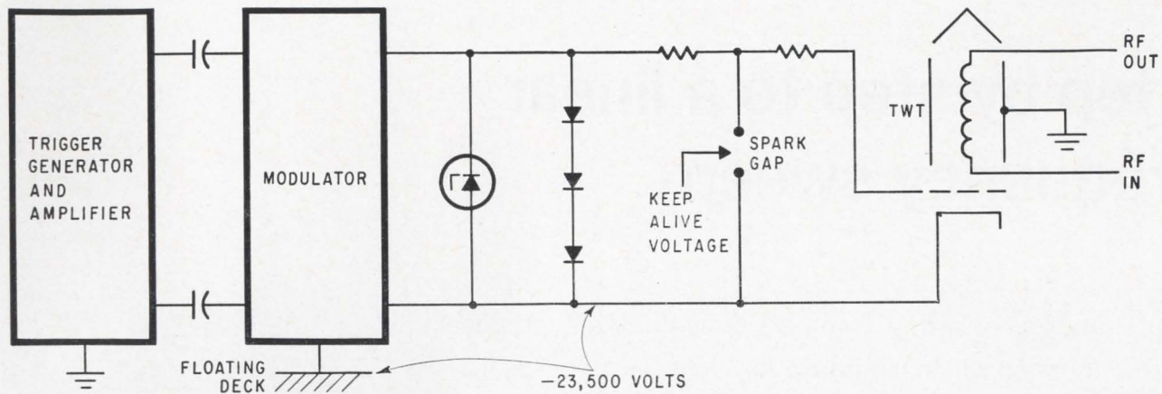
Modulator of floating deck at cathode potential is protected by spark gap. When gap breaks down, entire modulator circuit is at same potential. A crowbar across cathode power supply (not shown) protects twt by diverting arc current.
