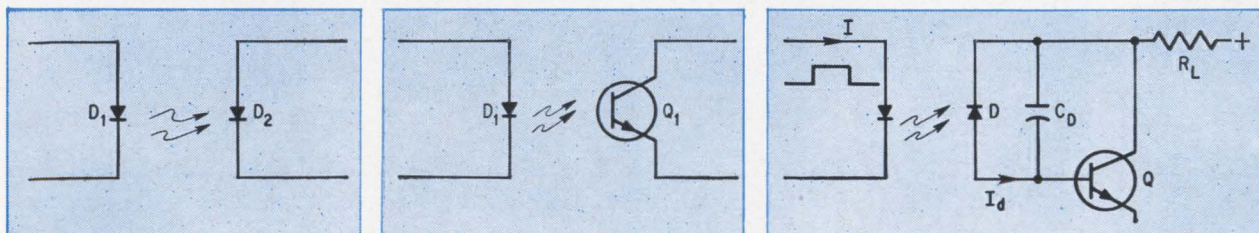
A light source ( D_1 ) optically coupled to a silicon photodetector ( D_2 ) is shown in the diagram at left; the detector photocurrent is very small compared to the current flowing in the source circuit. In center diagram, a phototransistor ( Q_1 ) provides an output current equal to the original current in the source circuit; but its equivalent circuit (right) has a large time constant, approximately R_L C_D times the transistor beta. This restricts the bandwidth capability.
