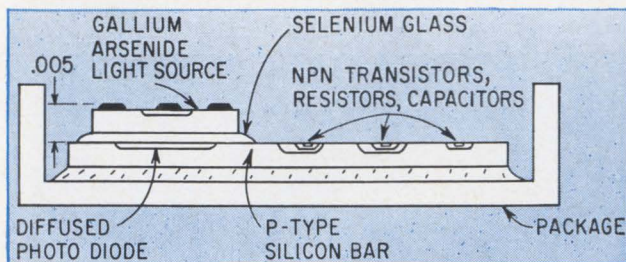
Cross-sectional diagram of the integrated circuit shows how the GaAs light source is positioned above the photo-detector diode. The addition of the light source and the selenium glass layer add only 0.005 inch to the height of the structure.
