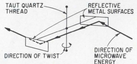
Microwave measuring instrument being designed by the National Bureau of Standards to provide absolute readings above 100 gigacycles.
