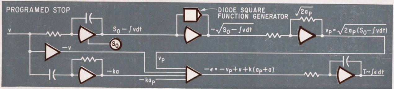
Analog computer for speed control, in simplified form, as used by General Railway Signal system.
