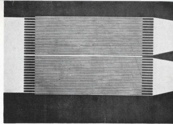
One way. Stanford University built this unidirectional surface wave transducer of lithium niobate.
