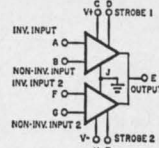
5711 High Speed Dual Voltage Comparator
