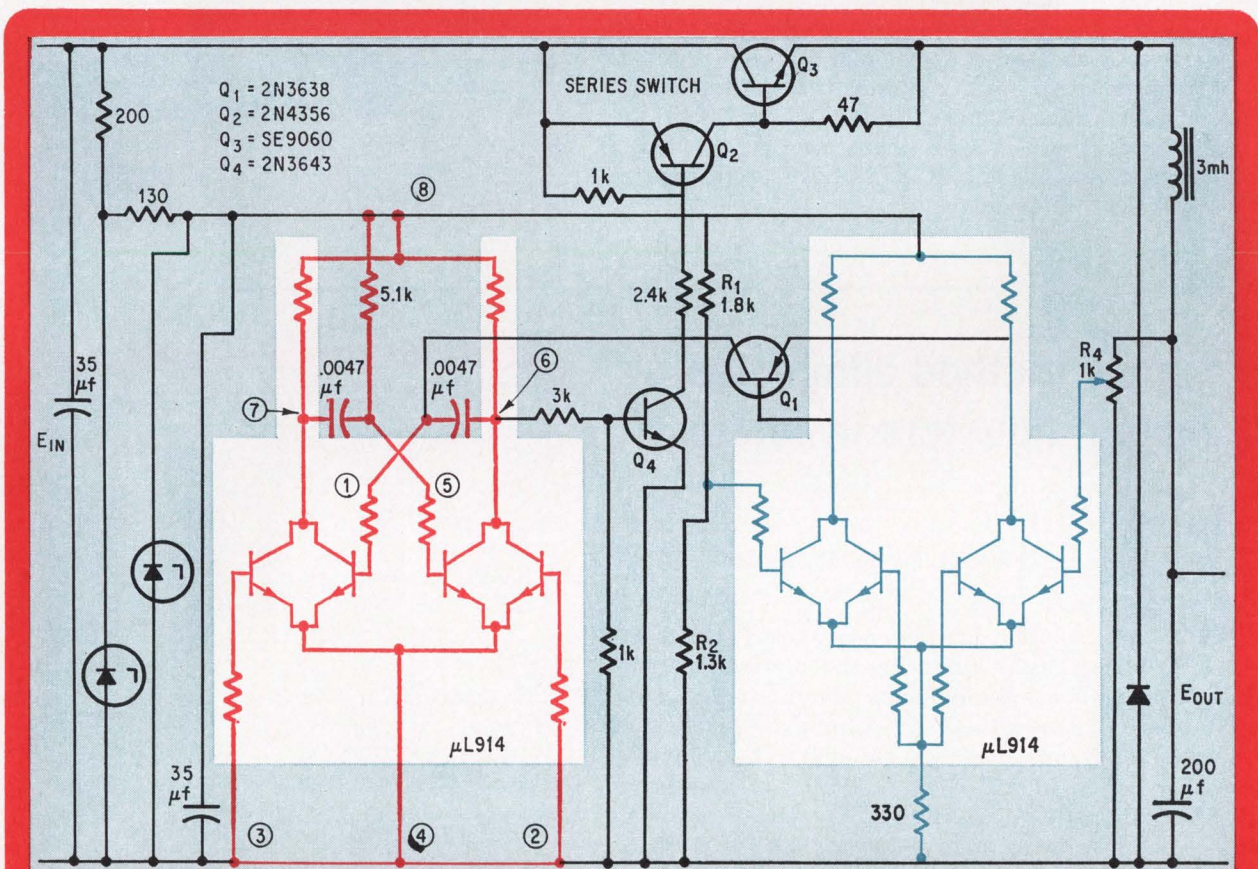
Versatility. With a few extra components, the uL 914 two-input dual AND gate can be converted into a differential amplifier and an astable multivibrator. Connecting the two makes a voltage regulator. The amplifier acts as an error detector, changing the duty cycle of the multivibrator.
