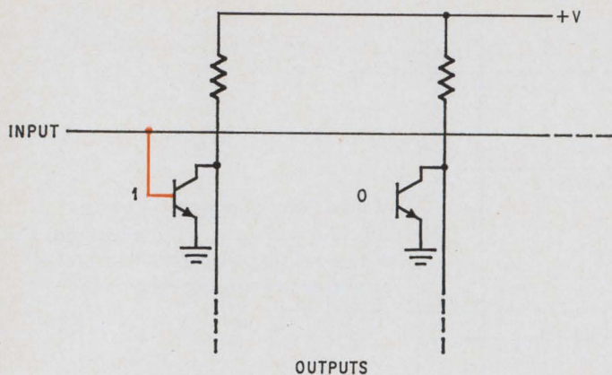
Bipolar array. A read-only memory can have bipolar transistors as its storage elements if the presence or absence of a base connection corresponds to 1's and 0's.
