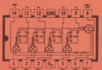
SN54/74L95 4-Bit Universal Shift Register
