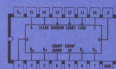
SN54/74192 Synchronous Up/Down Decade Counter
