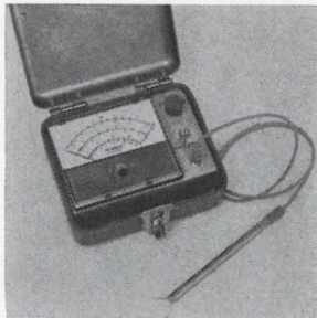
R-f voltmeter model 500 covers the frequency range from 20 khz to 500 Mhz with a voltage range from 200 mv to 15 v rms. From 20 khz to 100 Mhz, measurements are accurate to 3% of full scale; from 100 to 200 Mhz, accuracy is 5%; and from 200 to 50 Mhz, voltages are read from a calibration curve. High Frequency Engineering Co., 2626 Frontage Rd., Mountain View, Calif. [367]
