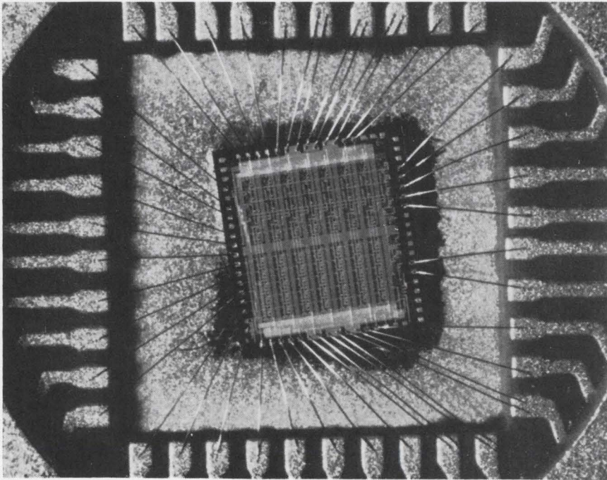
80-gate ECL. Packaged Philco-Ford chip contains 80 gates, which operate at speeds of 0.6 to 0.7 nanosecond at 7 to 10 milliwatts of power.
