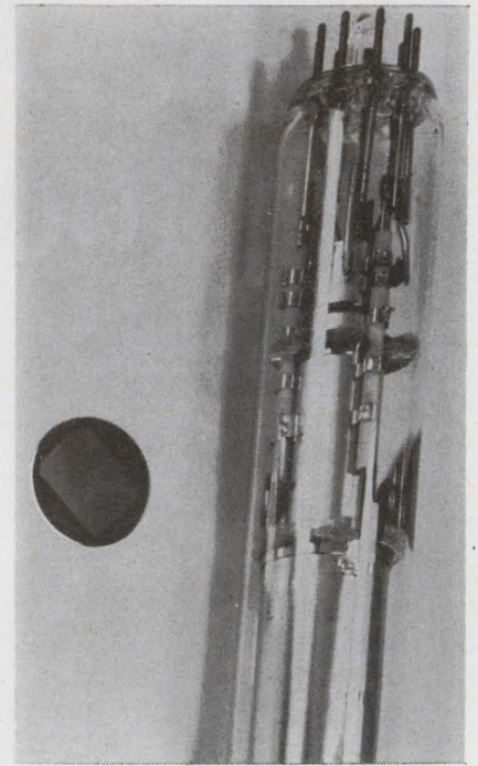
Sensor. Tube's target array, left, contains up to 750,000 diodes.
