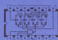
SN54/74L93 4-Bit Binary Counter
