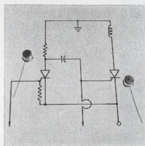
Power gate turnoff RTGD02 uses planar technology. It offers turn-off gain greater than 10 at 5 amps without sacrificing on-triggering sensitivity. Typical turnoff time at 5 amps is 2 \mu sec. The series is specified for operation to +125°C and is available in ratings from 60 to 400 v; it can withstand surges to 60 amps. Transistron Electronic Corp., 168 Albion St., Wakefield, Mass. [438]
