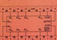
SN54/74L91 8-Bit Shift Register
