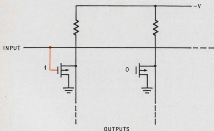
MOS FETs. As with bipolar transistors, at top of page, an array of MOS transistors can store data by a gate connection.
