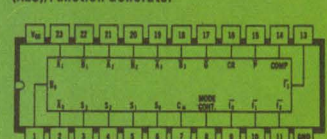
SN54/74181 4-Bit Arithmetic Logic Unit (ALU)/Function Generator
