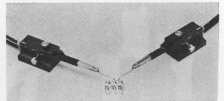
In place. Probes are held to bench by a vacuum as they test resistance values on circuit.
