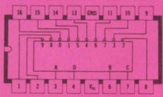
SN74141 BCD-to-Decimal Decoder/Driver
