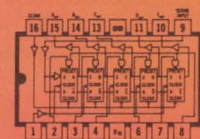
SN54/7496 5-Bit Shift Register (Dual Parallel-In, Out)
