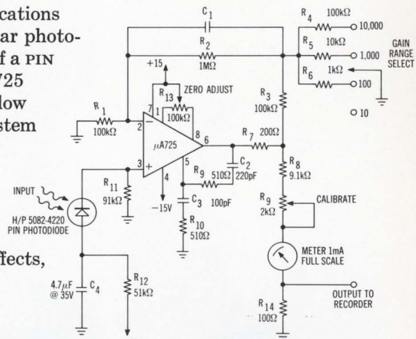
DC GAINS = 10,000, 1,000, 100, AND 10 BANDWIDTH = DETERMINED BY VALUE OF C_1 GAIN ACCURACY \times 1000 0.03% \mu A725 PIN PHOTODIODE AMPLIFIER
