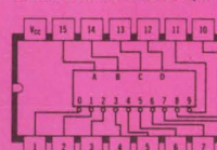
SN54/7445/145 BCD-to-Decimal Decoders/Drivers
