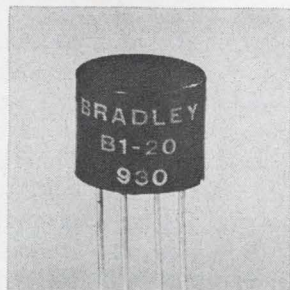
Encapsulated silicon bridge rectifiers series B1 are rated at 1.5 amps and are available in voltage ratings of 50 to 1,000 piv. They are intended for rapid insertion into p-c boards. Units save the user the time and expense of selecting and matching individual diodes for piv, forward voltage drop, and leakage current. Bradley Semiconductor Corp., 275 Welton St., New Haven, Conn. [441]
