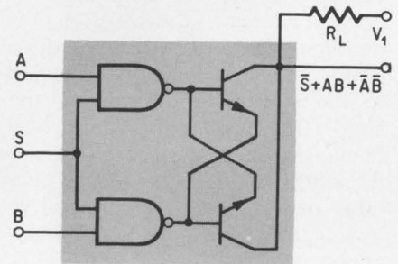
GATED COMPARATOR
