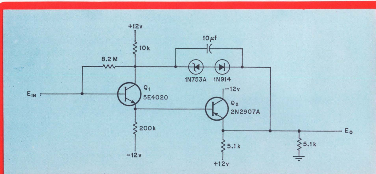
Low frequency. The zener diode bootstrap extends the operating range of the Darlington amplifier to d-c. Input capacity is reduced to 0.5 pf from the common 5 pf. With super beta transistors, input impedances in the 100-megohm range can be achieved, while the zener diode protects the transistors from breakdown.
