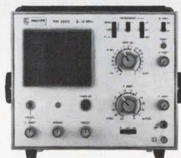
PM 3200 10MHz 2mV/div $480
