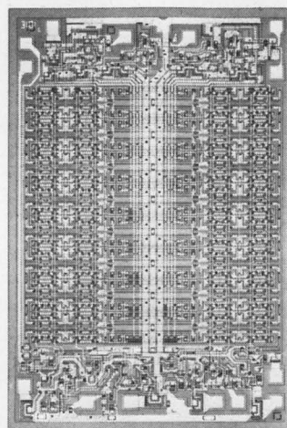
Model 3101 , a 64-bit bipolar RAM with 60 ns maximum access, drops in price by 38% to 60%.
