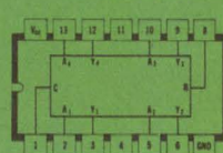
SN54/74H87 4-Bit True/Complement Element
