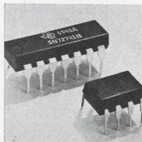
Operational amplifier IC designated SN72741 is short-circuit protected, and the internal frequency compensation provides high stability without the need for external components. High common mode input voltage and absence of latchup suit it for voltage follower applications. Power dissipation is typically 50 mw. Texas Instruments Inc., P.O. Box 5012, M/S 308, Dallas 75222 [442]
