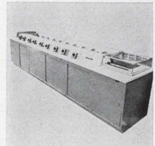
Automatic photomask developing system model 3100 is self-loading and unloading at beginning and finish of the process sequence. An adjustable timer at each tank allows independent time setting at each step. Once the process timers are set, the machine will automatically transfer the carriers from tank to tank. Fluoroware of California, 37433, Centralmont Pl., Fremont, Calif. 94536 [428]
