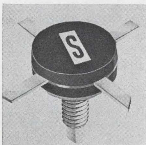
R-f power transistor SRD54117 can deliver 60 w output power at 150 Mhz with 28 v V_{CB} and a minimum 6 db gain. It can also deliver 50 w of output power at 175 Mhz with a minimum of 6 db gain. The device guarantees a 3:1 vswr capability. It is for use in vhf communications systems. Price (1-99) is $66. Solitron Devices Inc., 1177 Blue Heron Blvd., Riviera Beach, Fla. [440]
