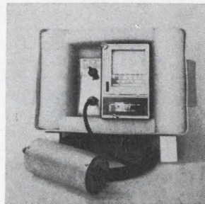
Transient recorder 111B has a self-contained probe detector and strip chart recorder for logarithmically displaying transients from 1 v to 1,000 v (60 db dynamic range) with no required scale adjustments. Frequency response of 50 khz is provided to compress transient data storage recordings by 100,000:1. White Electromagnetics Inc., Lofstrand Lane, Rockville, Md. [368]
