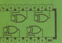
SN54/7486 Quad 2-Input Exclusive-OR Element
