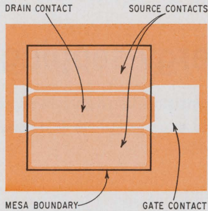
Competitive. Fairchild's new gallium-arsenide FET has a maximum frequency of oscillation over 12 Ghz.
