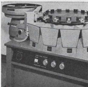
Transistor sorter type 1635 was developed to automatically test and sort T0-105 and T0-106 epoxy type transistors at a rate of 5,000 or more per hour. It automatically feeds components from a vibratory bowl via an orienting track to a 16-station index table which advances them to either a single or dual test probe. Daymarc Corp., 40 Bear Hill Rd., Waltham, Mass. [425]
