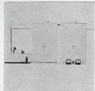
Dual oven will speed-dry photoresist on copper-plated through-hole p-c boards while limiting ring formation around the holes. Precision control of ring size is important in protecting the walls of the holes. The dual oven is conveyORIZED and consists of a hot-air impingement unit and a bench oven, with infrared heaters. Infra-Red Systems Inc., Route 23, Riverdale, N.J. [424]
