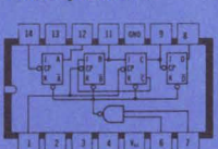
SN54/7492 Divide-by-12 Counter
