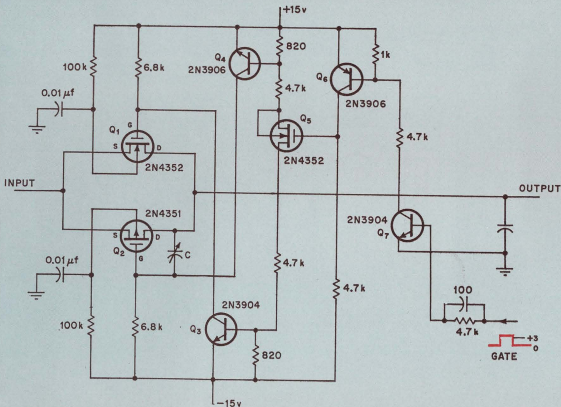
Throughput. The signal to be transmitted is fed to MOS FET's Q_1 and Q_2 simultaneously and transferred out when the two transistors are switched on. A positive pulse at Q_7 's input turns it on; in turn, Q_6 and Q_5 are switched on. Q_6 turns on Q_4 and Q_3 , which, in turn, bias the two MOS FET's into conduction.
