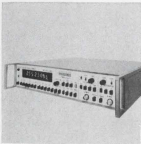
Digital counter/timer model 461 with 10 mv sensitivity measures frequency, period, multiple period, frequency ratio, multiple frequency ratio and time intervals, and totalizes. The standard configuration provides a counting rate of from d-c to 20 Mhz, and displays measured units on a seven-digit display with storage. Dynasciences Corp., 9601 Canoga Ave., Chatsworth, Calif. [366]
