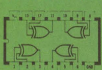
SN54/74L86 Quad 2-Input Exclusive-OR Element
