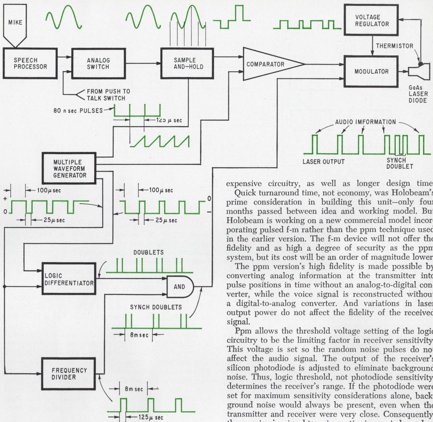
Light the light. Both the audio pulses out of the comparator and the synch doublets modulate the gallium arsenide laser diode on and off, corresponding to the input voice signal.
