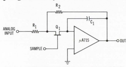
BASIC OPERATIONAL SAMPLE AND HOLD CIRCUIT
