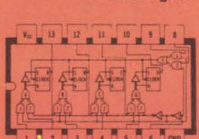
SN54/7495 4-Bit Universal Shift Register
