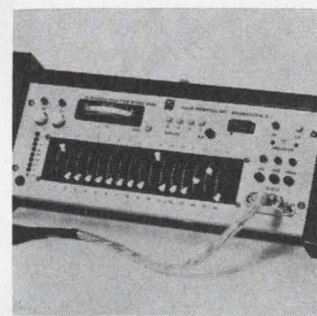
Versatile analyzer model 2080 is for testing IC's and modules. It contains a built-in stimulator-generator, monitor, and IC power supply, and eliminates the need for any peripheral test instrumentation. The internal power supply provides 3 to 7 v for energizing chips or modules under test. Model 2080 is 16 x 10 x 6½ in. Pulse Monitors Inc., 351 New Albany Rd., Moorestown, N.J. [364]
