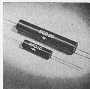
High-voltage silicon rectifiers series RCD-RFD have a piv of 8,000 to 45,000 and a recovery time of 300 nsec. They are rated at a forward current of 20 ma. Applications include power sources of crt's, data displays, radar displays, and r-f supplies where h-f sine-wave, square-wave or pulse inputs are used. Electronic Devices Inc., 21 Gray Oaks Ave., Yonkers, N.Y. [443]
