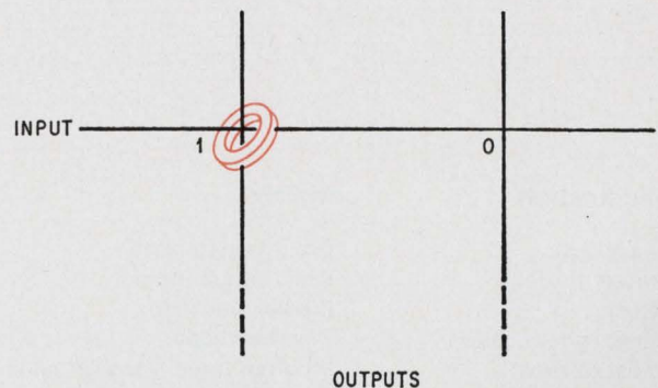
Old-timer. A toroidal transformer at each intersection corresponding to a 1 is perhaps the oldest form of read-only memory, but the array is handmade and thus expensive.
