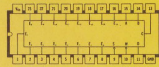
SN54/74150 16-Bit Data Selector
