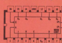
SN54/74L99 4-Bit Universal Shift Register
