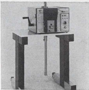
Mini-Charger 8014 is a manually operated handler that conditions IC's through an environment of -65^{\circ} to +150^{\circ}\text{C} . Easily accessible test contactors can be interchanged within 5 minutes to permit handling of T0-5, short and long lead, dual in-line pack, and flatpack devices, in carriers, in an environment of \pm\frac{1}{4}^{\circ}\text{C} at the test contactor. Delta Design, Box 1118, La Mesa, Calif. [421]
