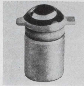
Phototransistors type OP300 will generate light currents in excess of 12 ma at irradiance of 1 mw/cm 2 . With normal light input, the current output is sufficient to function as an IC-logic circuit driver. Units are built in a package that may be mounted on 0.087-in. centers and are suited for IBM system 3 minicard uses. Optron Inc., 1201 Tappan Circle, Carrollton, Texas [438]
