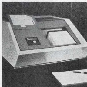
Card reader SR-600 maintains a rate of 600 80-column cards each minute or 750 51-column cards each minute. As an intermediate speed card reader, it comes as a table unit offering simplicity of operation. Unit weighs 125 lbs, has a hopper capacity of 1,400 cards and a stacker capacity of 1,000 cards. Data Products Corp., 6219 DeSoto Ave., Woodland Hills, Calif. [406]
