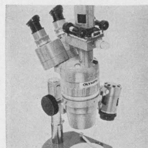
Hybrid-circuit production and inspection time is cut 50% by a new stereo-microscope system. The Infoscope projects circuit diagrams, waveforms or digital displays into the bonding operator's or inspector's field of vision. This permits checking assembly accuracy and performance without looking away from the eyepieces. Olympus Corp of America, Nevada Dr., New Hyde Park, N.Y. [428]
