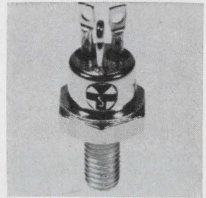
Power transistors JAN 2N2880 and JAN TX 2N2880 are npn silicon triple-diffused devices for power amplifiers and switching uses. Features include: 30 w dissipation capability, low leakage current, 20 Mhz minimum gain cutoff, and low drive requirements. Units are suited for use in h-f inverters and converters. Silicon Transistor Corp., East Gate Blvd., Garden City, N.Y. [443]
