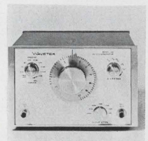
Function generator model 142 features a frequency range of 0.001 hz to 10 Mhz and an asymmetry function. It provides positive- and negative-pulse outputs as well as the usual sine, square, and triangle waveforms. Output frequency can be controlled manually, or by applying a control voltage to the front panel BNC connector. Wavetek, P.O. Box 651, San Diego, Calif. 92112 [3681]
