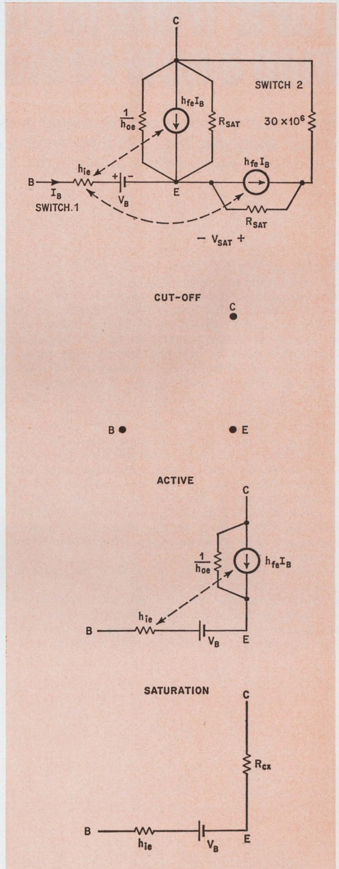
Switching. The three-region model used in ECAP simulates a transistor that changes regions of operation during the analysis. Ideal switch permits the use of a piecewise linear model.
