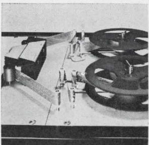
Paper tape spooler accommodates 5-8-track paper or mylar tape at bidirectional speeds to 1,000 characters/sec and rewind speeds to 1,000 characters/sec. The high reliability and ruggedness is suited for numerical control, ground support systems, test equipment, digital data handling, and computer input. Datascan Inc., 1111 Paulison Ave., Clifton, N.J. 07013 [405]
