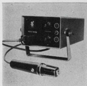
Rotary thermal wire stripper model RT-1 features centrifugal-force insulation severing that ends conductor damage. It will strip most insulations used in electronics manufacturing including Teflon and Kapton without damage to even hair-like No. 40 strands. Wire diameters are No. 40 to 0.300 in. Roto-Therm Division, Republic Corp., 950 N. Sepulveda Blvd., El Segundo, Calif. [425]
