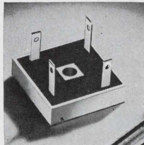
Single-phase, silicon-bridge rectifier model XP409 is for p-c use. Units measure 1 in. square by ¼ in. high, yet are rated for 15 amp resistive - inductive loads. Characteristics at 60 hv include: 8 piv ratings from 100 to 800 v with maximum inputs from 70 to 560 v rms, and a surge current rating of 240 amps max. Sarkes Tarzian Inc., 415 College Ave., Bloomington, Ind. [442]
