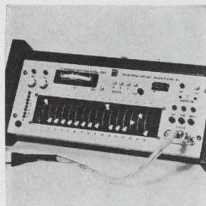
Compact IC/module analyzer model 2080 contains a built-in stimulator, generator, monitor and IC power supply, and eliminates the need for any peripheral test instrumentation. It will test chips with up to 16 pins. Unit measures 16 x 10 x 6½ in., and weighs 16 lbs. It is priced at $1,290 in small quantities. TeleSciences Inc., 351 New Albany Rd., Moorestown, N.J. 08057 [3621]
