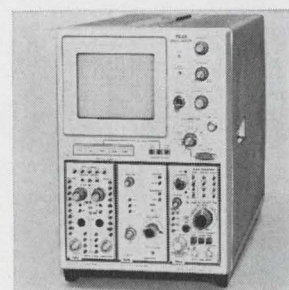
Flexible oscilloscope type 7503 is a 90-Mhz, three plug-in unit with a dual-trace vertical amplifier in the mainframe provided by vertical-mode switching, which enables the user to simultaneously measure waveforms with widely different characteristics by electronically switching between two vertical plug-ins. Tektronix Inc., P.O. Box 500, Beaverton, Ore. 97005 [3661]
