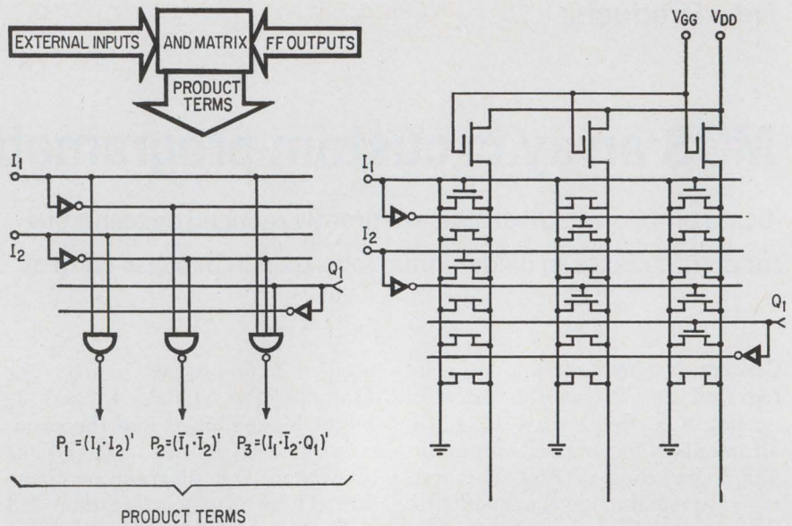
Product matrix. External inputs such as I_1 and I_2 and flip-flop outputs such as Q_1 are combined in the product matrix to form products such as P_1 , P_2 , and P_3 . To connect signals according to the required logic program, metalization forms gates of MOS transistors as shown at right.
