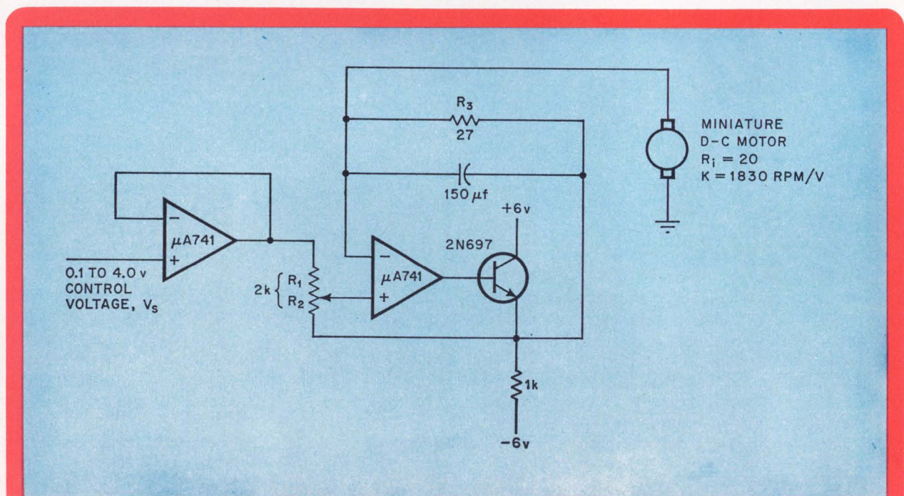
Negative impedance. The equivalent resistance of the motor's driving source is made equal to the negative of the motor's internal resistance thereby rendering the motor's speed independent of load variations. The negative impedance is measured at the op amp's negative terminal with respect to ground.
