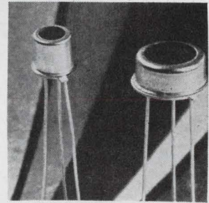
Silicon photodiode SGD-0404 is suited to a variety of applications including: card and tape readers, process control, and remote switching. Typical characteristics include: sensitivity of 0.5 amp/watt at 0.9 micron; spectral-response range from 0.35 micron in the UV to 1.13 microns in the near IR; rise time less than 1 nsec. EG&G Inc., 160 Brookline Ave., Boston [439]
