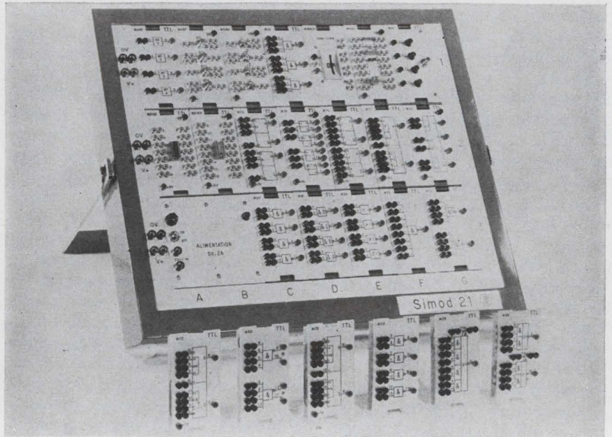
Very simulating. Integrated circuit breadboard holds modules for each different IC type. Patch cords interconnect modules and power supply.
