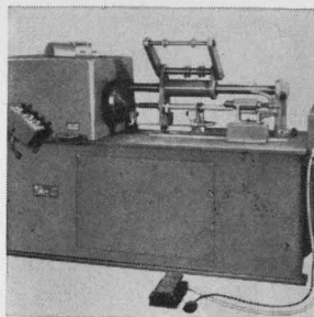
Gearless, heavy duty, multiple transformer winder model 500-AM features instant spiral/rapid traverse, wire size range 10-28 Awg, 14 in. max. coil o-d, 12 in. max. coil length, 30 in. max. loading distance for multiple winding, 8-75 turns-per-in. winding range, 0-to-250-rpm winding speed. Price is $8,600; delivery, 8-10 wks. Geo. Stevens Mfg. Co., 6001 N. Key-stone Ave., Chicago [423]
