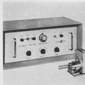
Automatic pressure controller series 213 provides increased yield and better reproducibility from run to run in sputtering and reactive evaporation processes. Steady pressure control of doping gases makes it useful in preparation of semiconductors. Control has been achieved from above 1 atmosphere to less than 10 -11 torr. Granville-Phillips Co., E. Arapahoe Ave., Boulder, Colo. [424]
