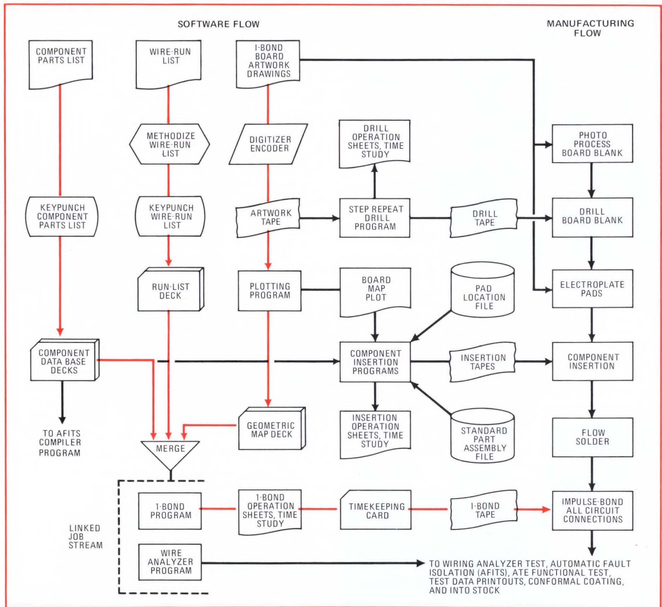
5. Computer-aided manufacturing. Software for board drilling, component insertion, interconnection, testing and time studies are under direct computer control in this process. Colored lines highlight inputs that control the final impulse-bonding step.
