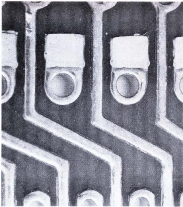
1. I-Bond pads. On impulse-bonded circuit boards, bonds are made directly to the rectangular area of the pads, shown magnified here 10 times. Components are mounted and wave-soldered in the plated-through holes beside the pads.
