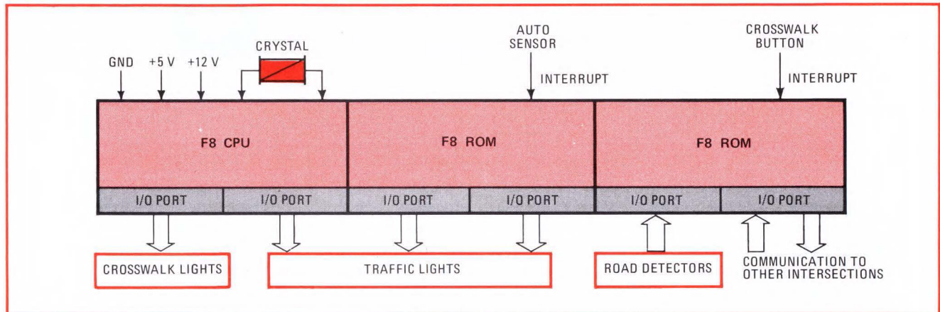
5. Versatile. As a traffic-light controller, one F8 CPU and two F8 ROMs can count passing autos, provide a pedestrian crosswalk interrupt input, and also time the traffic-light changes. An external crystal precisely sets the clock frequency.
