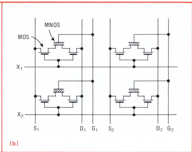
6. Two types of RAM cells. Cell belonging to Intel's ECL-compatible 4,096-bit 80-ns memory is a four-transistor dynamic type made static-like with charge pumping (a). Toshiba MNOS cell has nitride gates for nonvolatile operation (b) but requires a writing voltage of -35 V.
