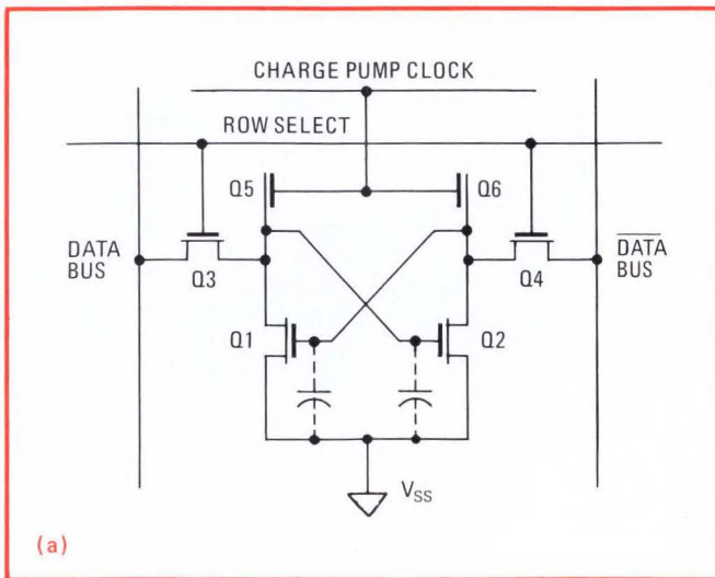
6. Two types of RAM cells. Cell belonging to Intel's ECL-compatible 4,096-bit 80-ns memory is a four-transistor dynamic type made static-like with charge pumping (a). Toshiba MNOS cell has nitride gates for nonvolatile operation (b) but requires a writing voltage of -35 V.
