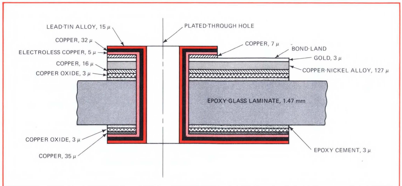
2. Pad cross section. Normal printed-circuit laminating, etching and photoplatting processes are used to deposit an I-Bond pad on an epoxy-glass board. A special material is used for the pad—a copper-nickel foil alloy, which is impulse-bonded with a nickel wire.
