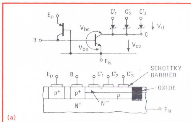
2. Schottky speed. Performance of injection-type gates is boosted by Schottky outputs. In Motorola's C 3 L gates (a) either a complementary pnp or resistor-limited current source can be used. In either case gate collapses to less than 13 mil 2 with passive isolation.
