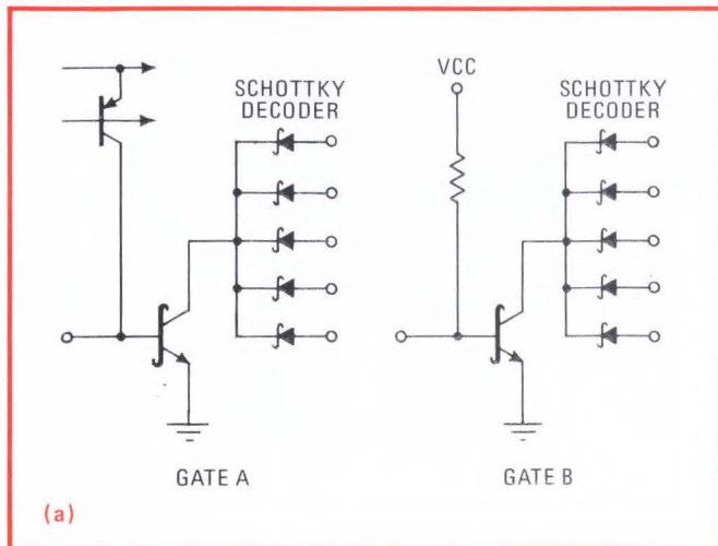
2. Schottky speed. Performance of injection-type gates is boosted by Schottky outputs. In Motorola's C 3 L gates (a) either a complementary pnp or resistor-limited current source can be used. In either case gate collapses to less than 13 mil 2 with passive isolation.
