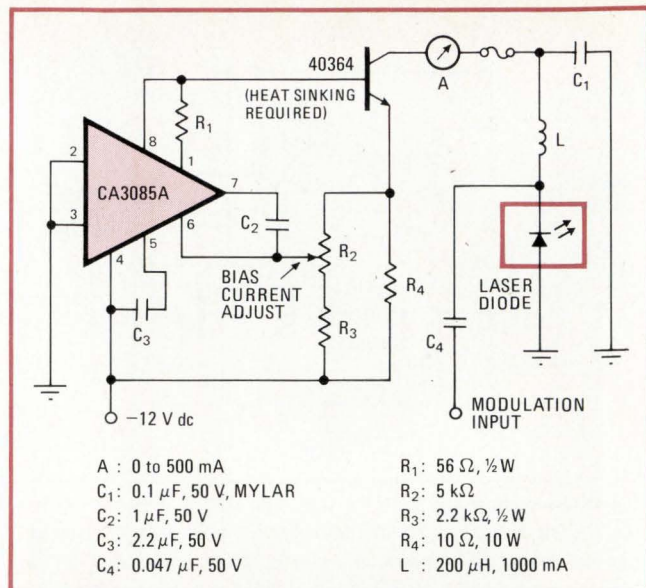
4. Measuring linearity. A 30-milliampere peak-to-peak 10-megahertz sine wave was coupled through capacitor C_4 to modulate the laser diode. The light output was measured, and the first harmonic was 40 dB below the fundamental.
