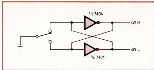
2. Switch-debouncing circuit. Part of a 7404 package debounces spdt switch. Signals are active when switch has position shown.
