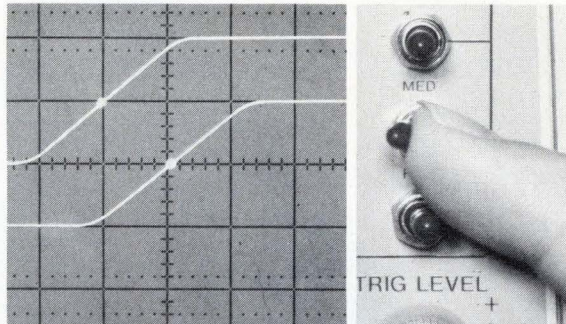
1. Position intensified markers (or adjust position controls for voltage measurements)
