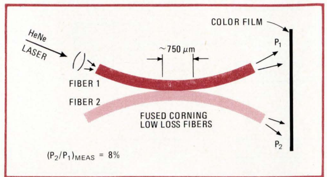
4. Mixing modes. One method of coupling light between single fibers is to bring the cores of the optical fibers so close together for a selected interaction length that the light modes of one fiber mix with those of the other fiber.
