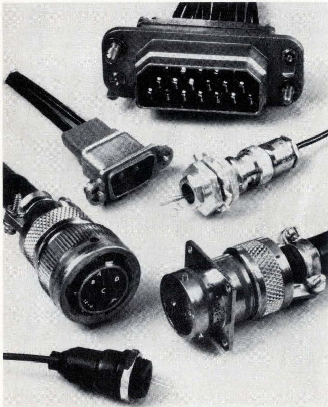
1. Wide selection. Connectors for fiber-bundle cables are available in both circular and rectangular shapes and can accommodate from 1 to 18 optical channels. These products can also couple either photodetectors or light sources to fibers.
