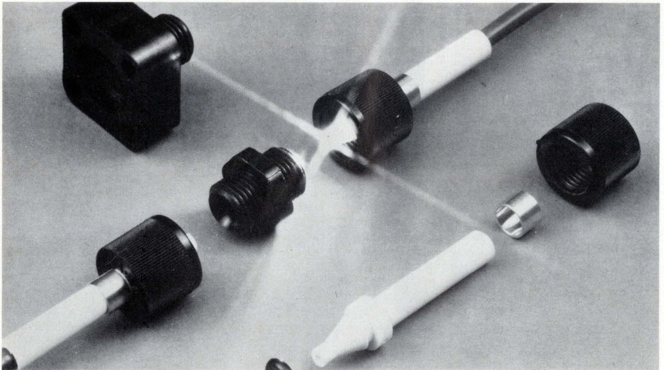
1. Plastic housing. This connector assembly can handle fiber bundles with diameters from 0.02 to 0.075 inch. The termination mates with a splice bushing for fibers (middle) or a bushing (top) that houses several standard light sources or detectors.
