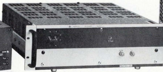
1000W Module Model CPS 15–50, unmetered Power Module shown with "ears" for 19" rack mounting. The ears are detachable for chassis mounting.
