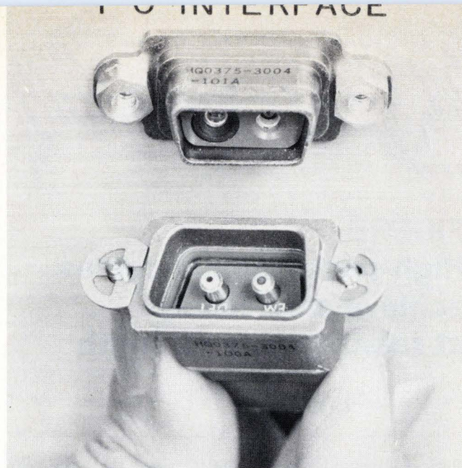
9. Two-way. The bulkhead side of Spectronics' optical-fiber plugable interface connector houses both the light-emitting-diode source and p-i-n photodiode detector needed to send and receive signals in a duplex fiber-optic transmission system.
