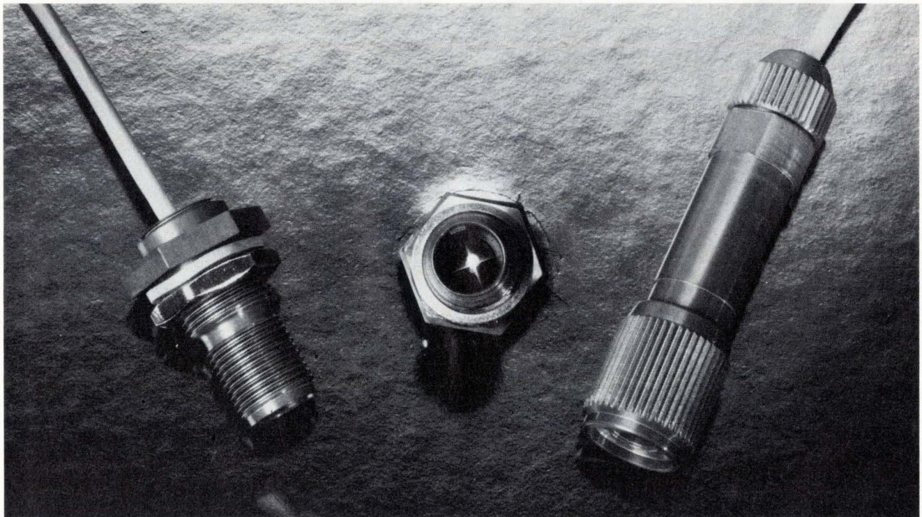
2. New entry. Few companies as yet are marketing single-fiber-per-channel connectors, but this recently released connector from ITT Cannon Electric can be used to join two single fibers or to couple a photo or a LED or laser diode to the fiber.
