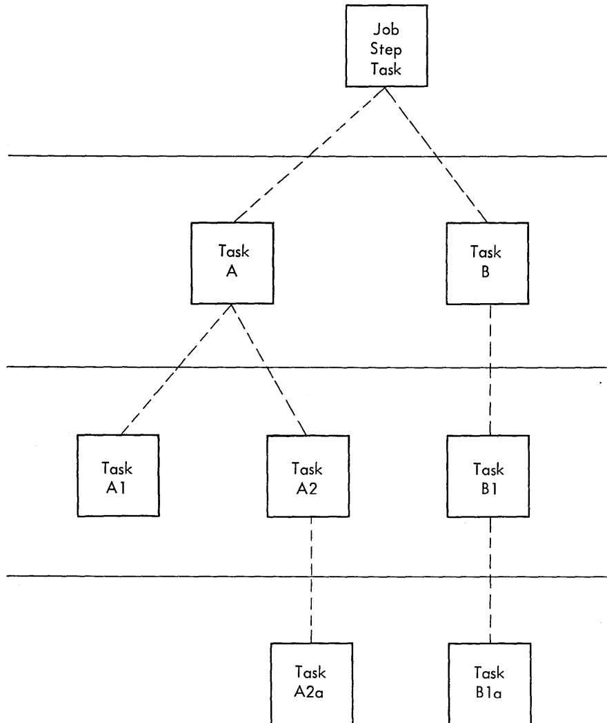
Figure 10. Task Hierarchy
