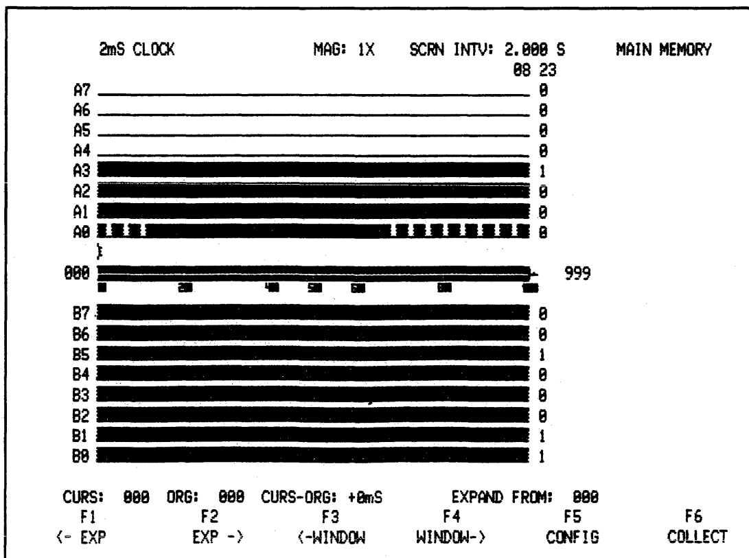
Figure 3-33. Timing Display At 1X Magnification
