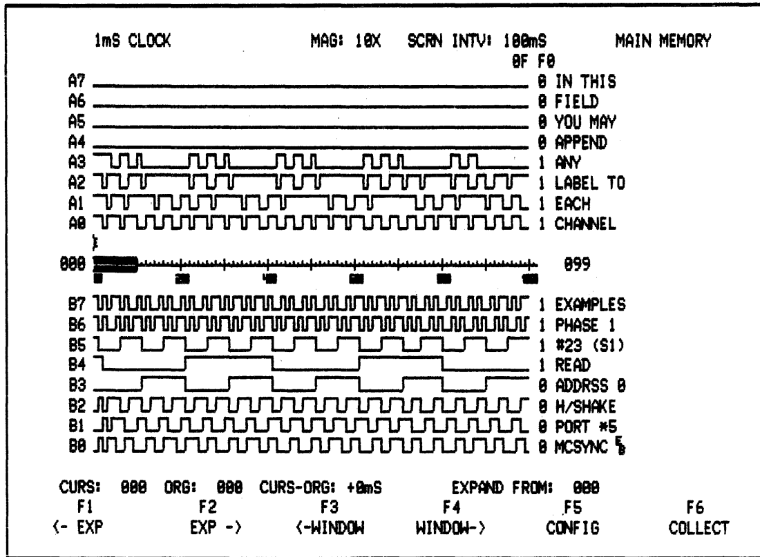
Figure 3-31. Timing Diagram Assignment of Labels (NAMES)
