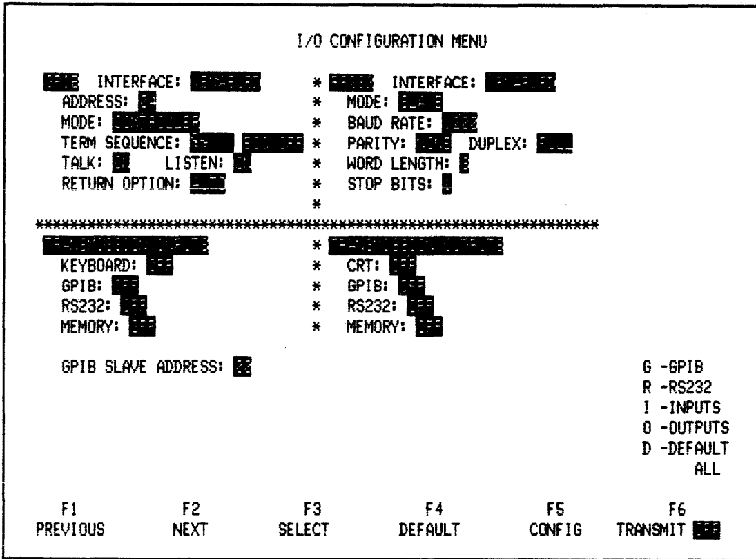
Figure 3-109. I/O Menu
