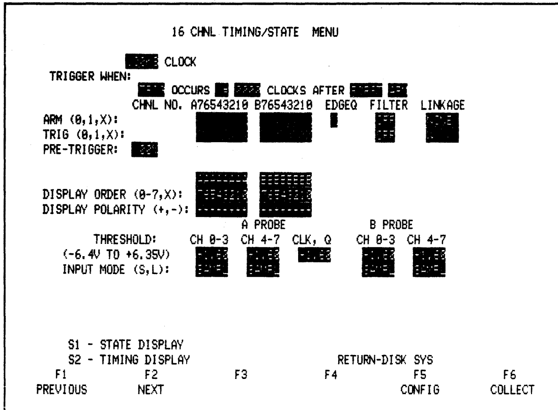
Figure 3-77. Timing Menu
