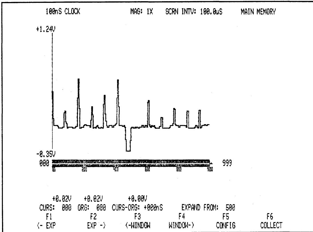
Figure 3-67A. Main Memory Displays
