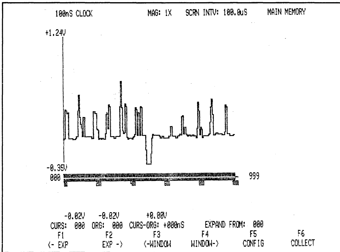
Figure 3-65. Video Signal At 1X Magnification
