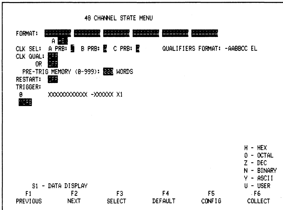
Figure 3-72. State Menu
