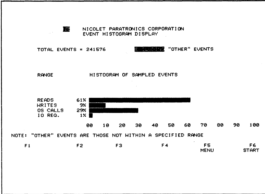
Figure 1-19. Event Histogram Bar Chart Display
