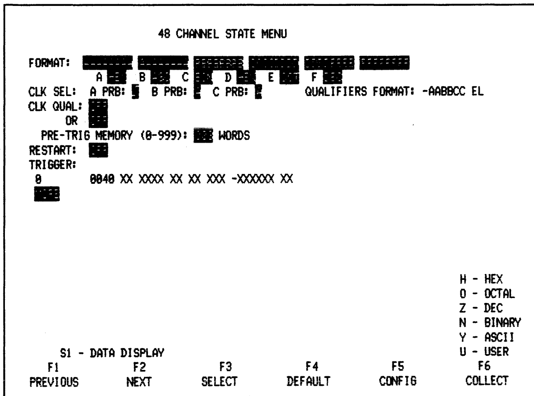
Figure 3-14. State Menu Set for Pretrigger Data Collection
