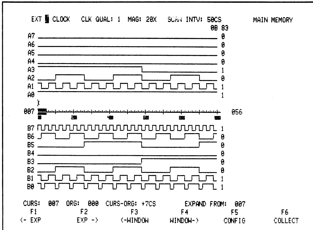
Figure 3-46. Timing Diagram Using An External Clock
