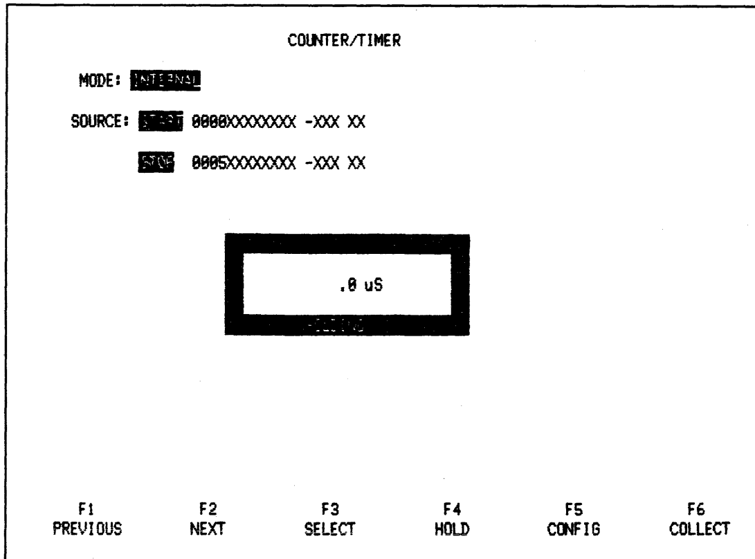
Figure 1-18. Measuring Interval Between Two State Events
