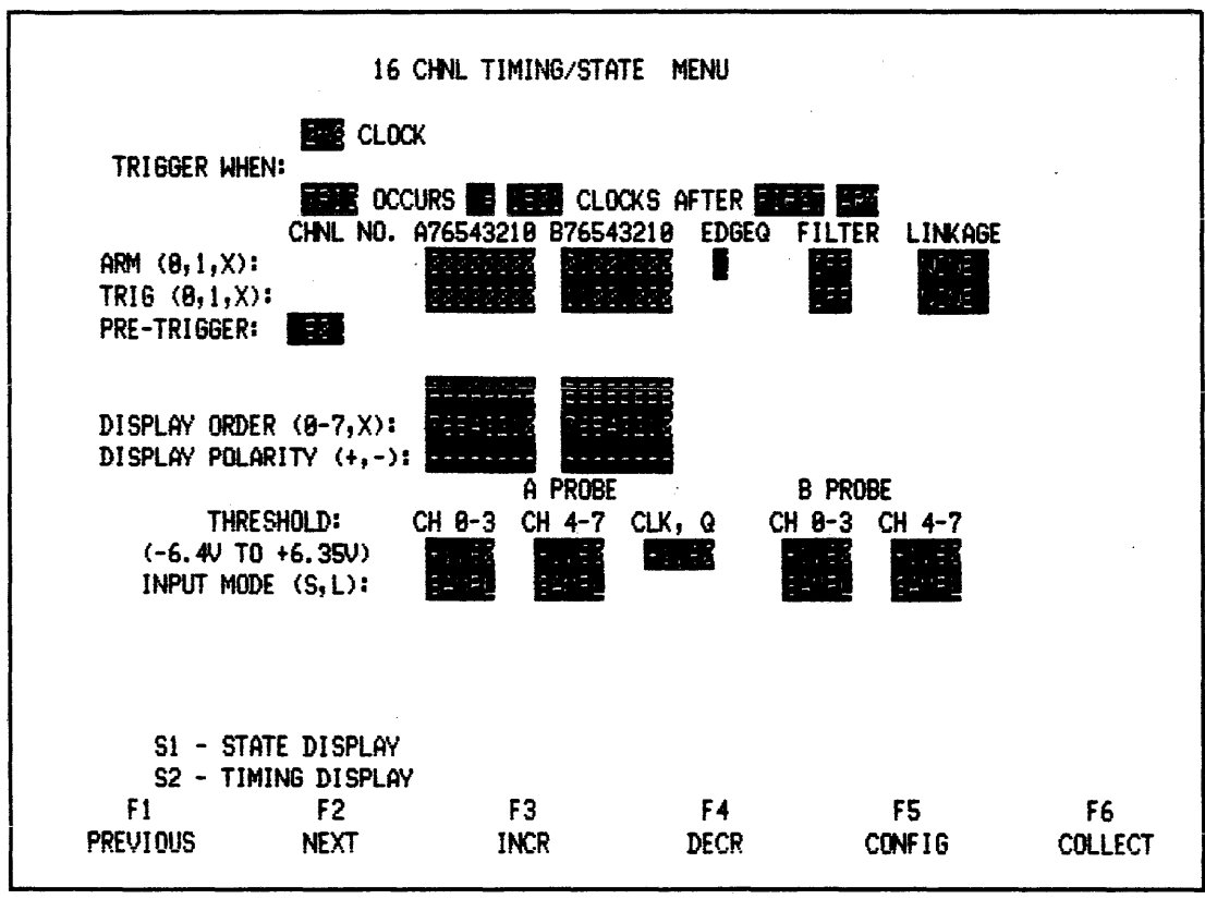
Figure 3-32. Menu Corresponding to This Example (Thus far)
