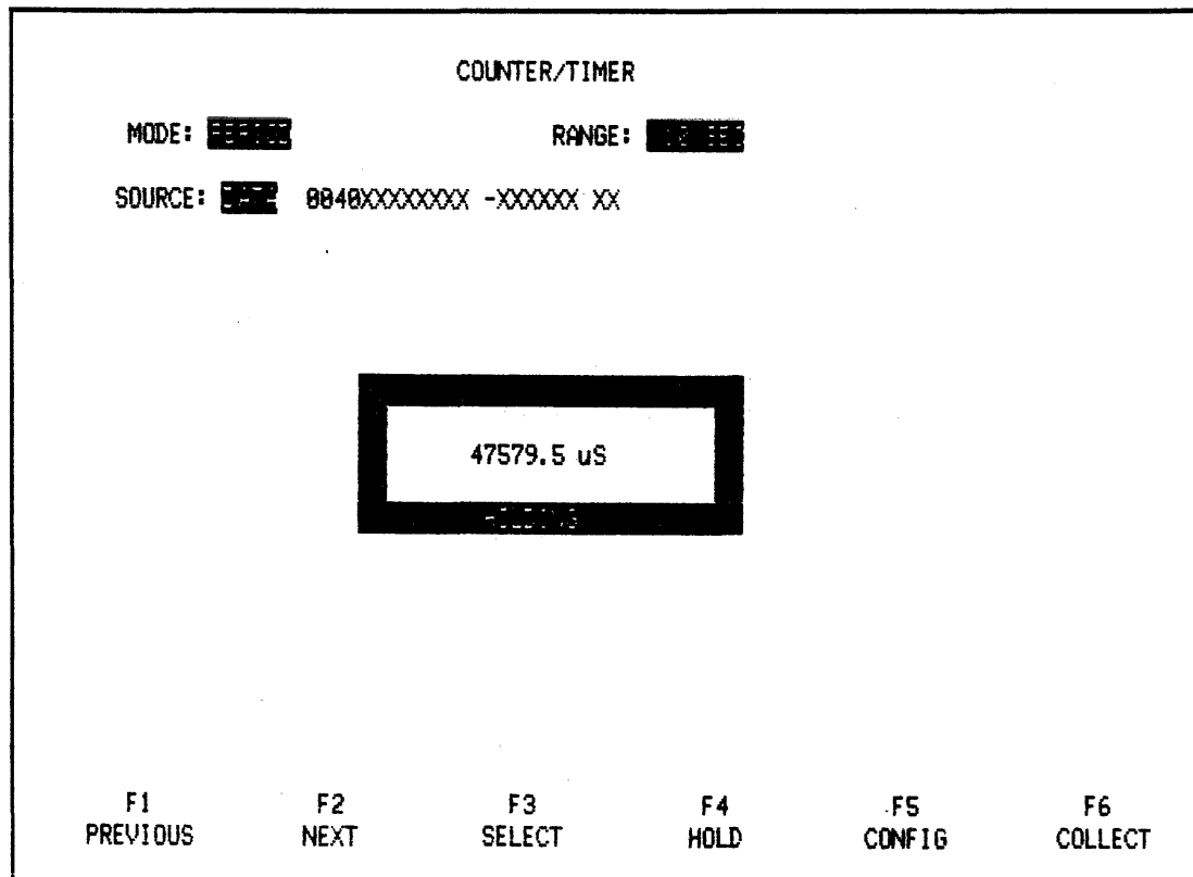
Figure 3-55. Period Measurement Using Counter-Timer
