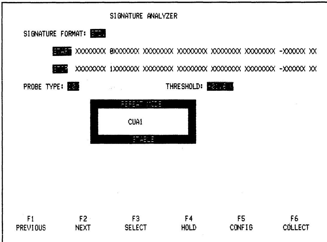
Figure 3-59. New Signature For DB0 (B Counter)
