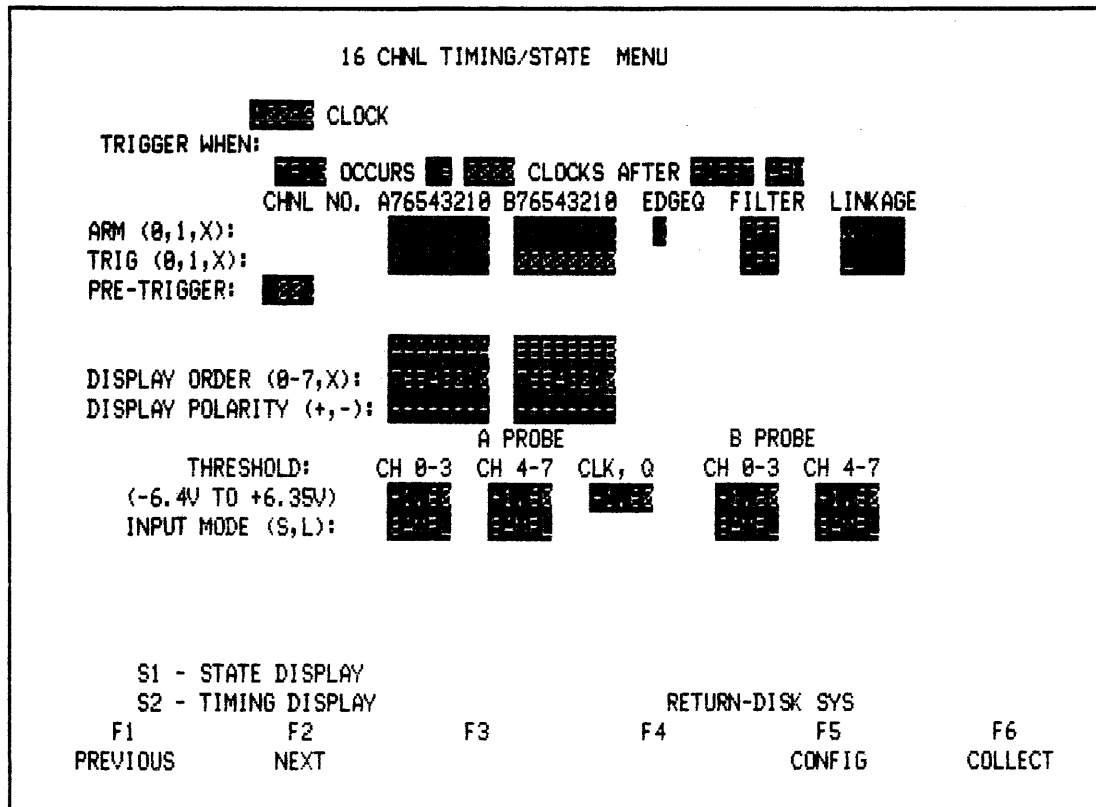
Figure 3-81. Timing Menu
