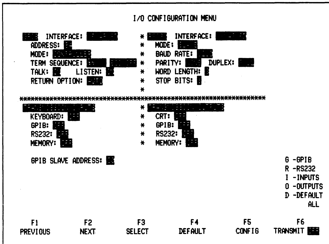
Figure 1-29. I/O Configuration Menu
