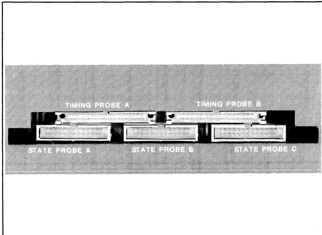
Figure 2-3. Probe Connections
