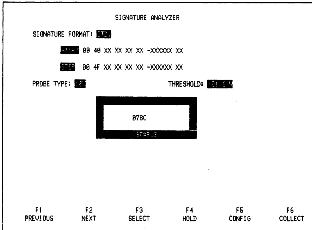
Figure 1-22. Signature Analyzer Menu For Developing Software Signatures
