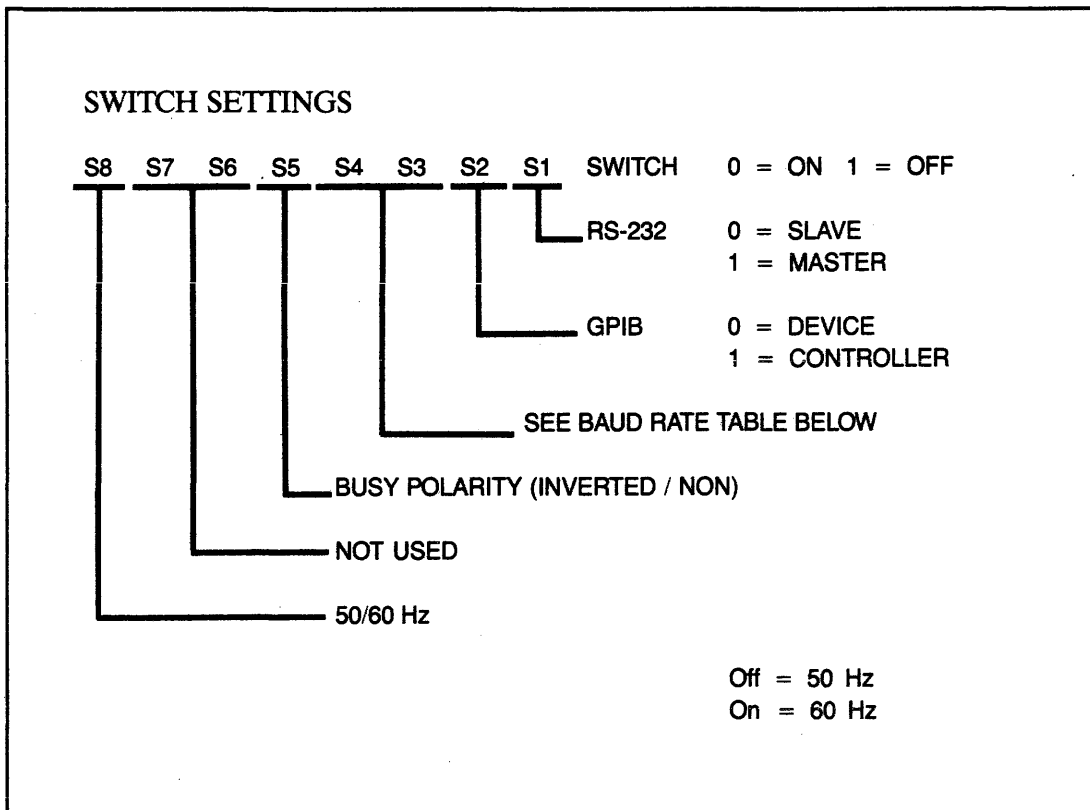
Figure 3-108. Processor Board DIP Switch Settings
