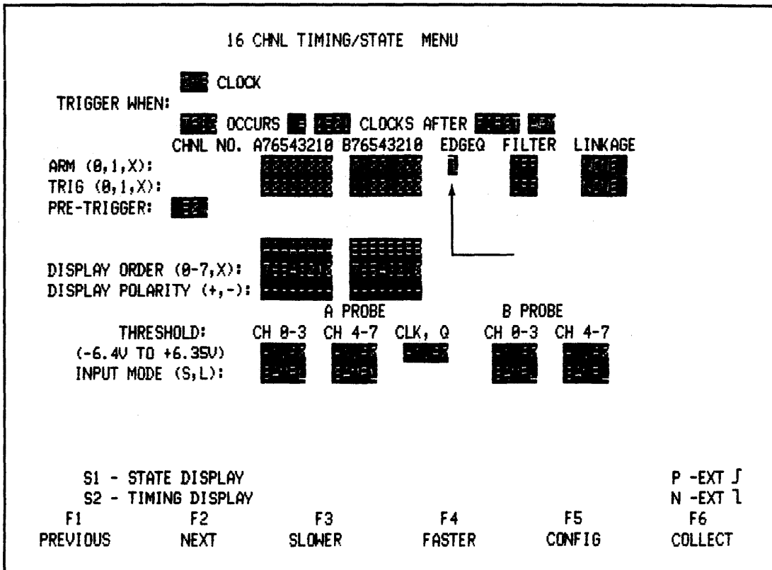
Figure 3-36. Position of Edge Qualification Field In Menu
